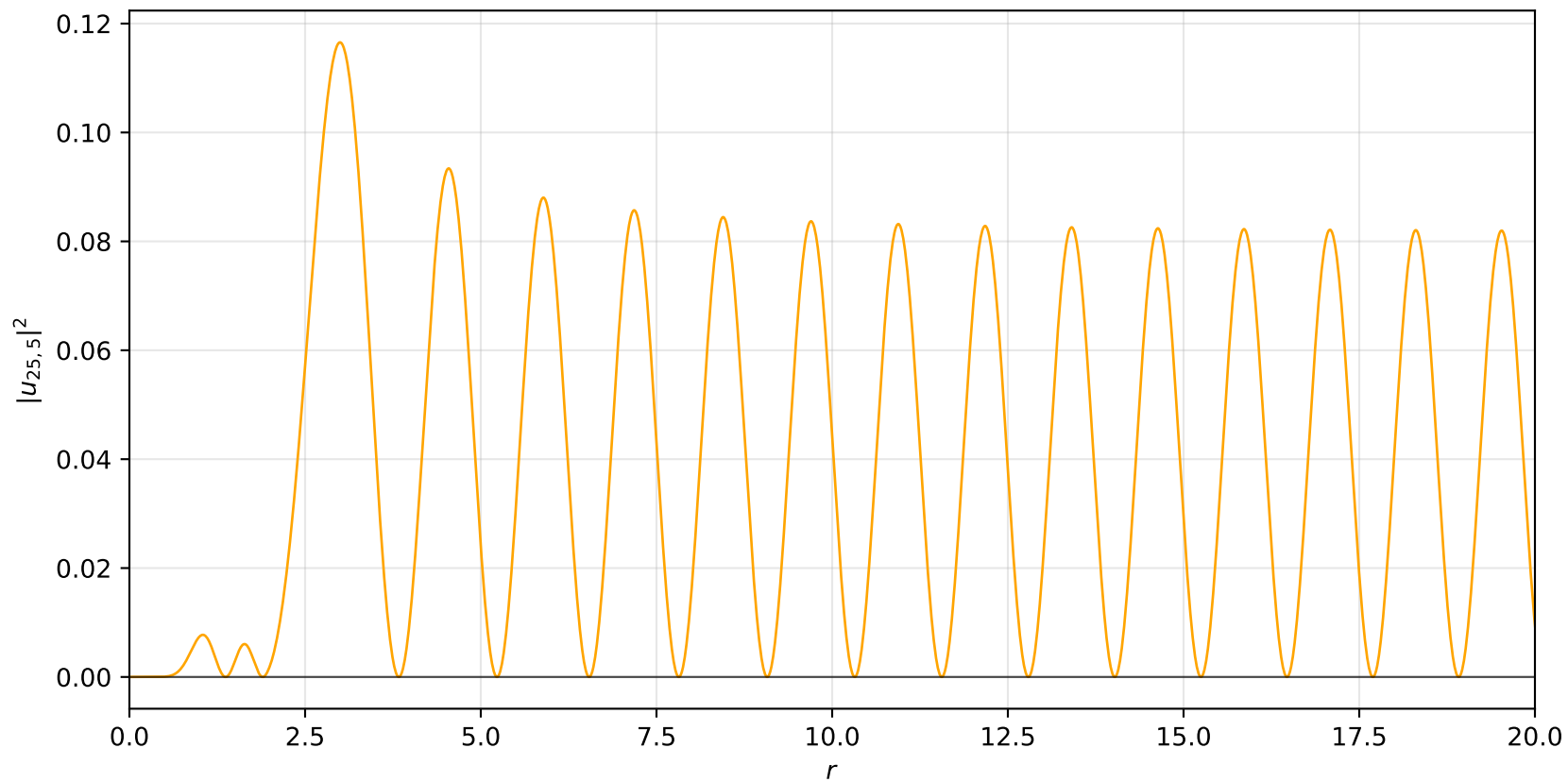
Probability Density: n = 25, \ell = 5
