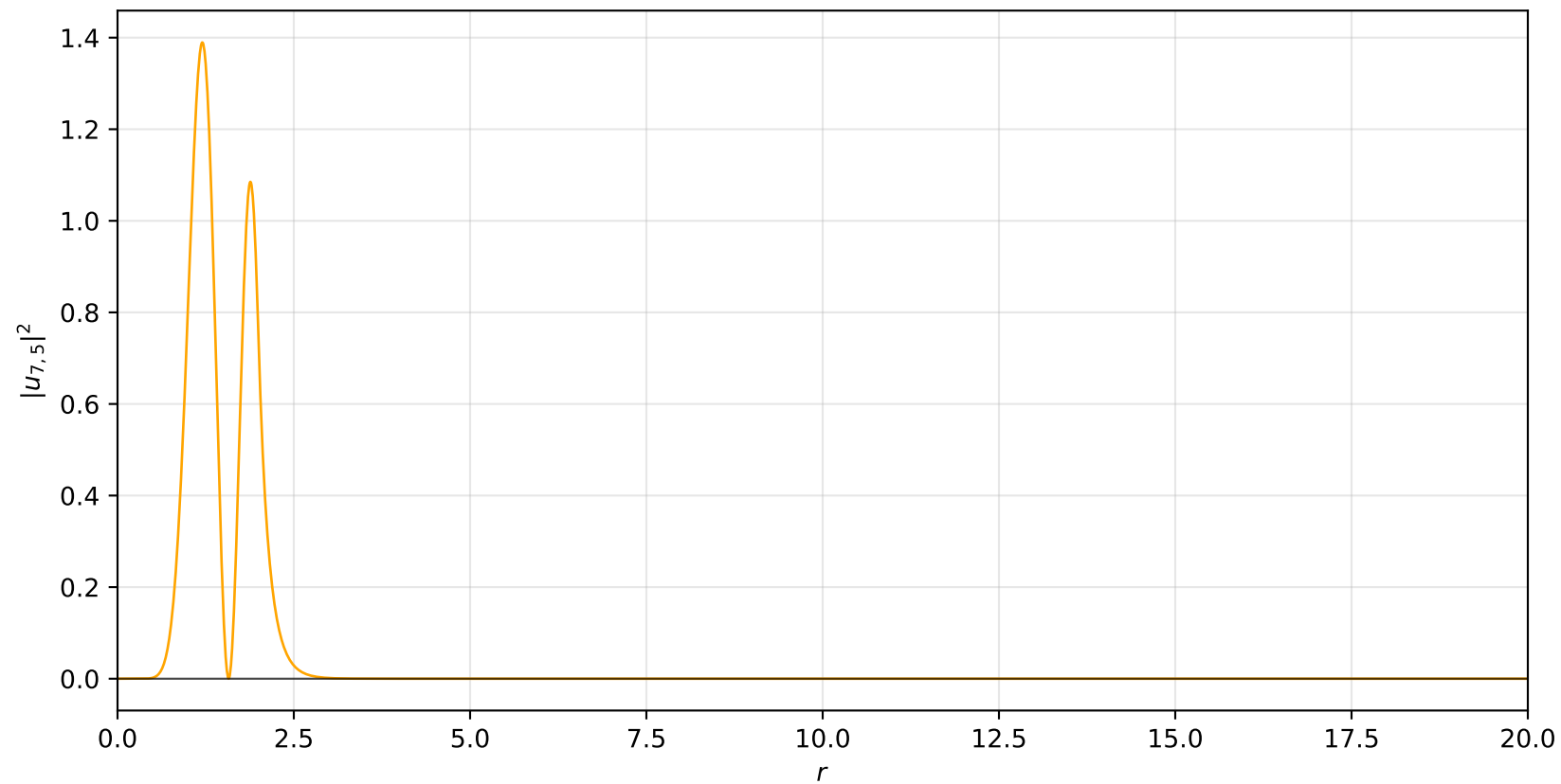
Probability Density: n = 7, \ell = 5
