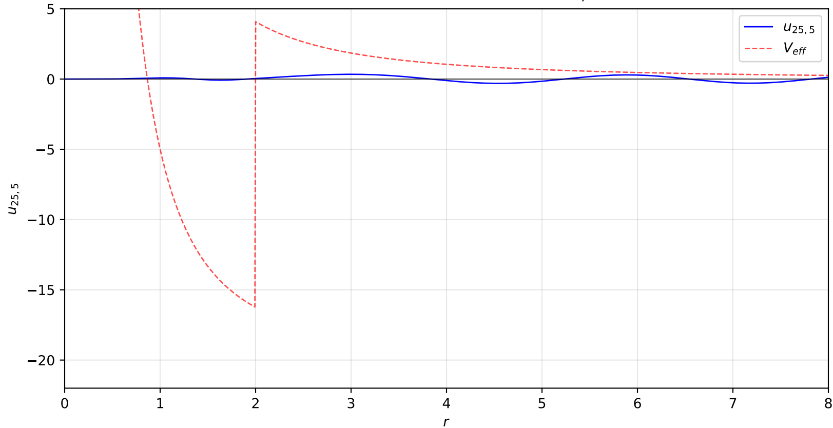
Reduced Radial Wave Function: n = 25, \ell = 5
