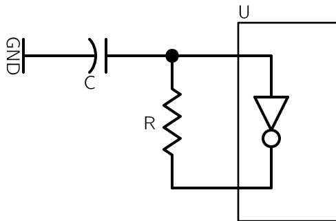
RC Oscillator
