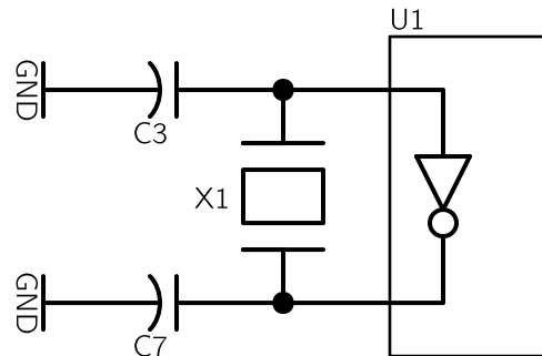
Pierce Oscillator
