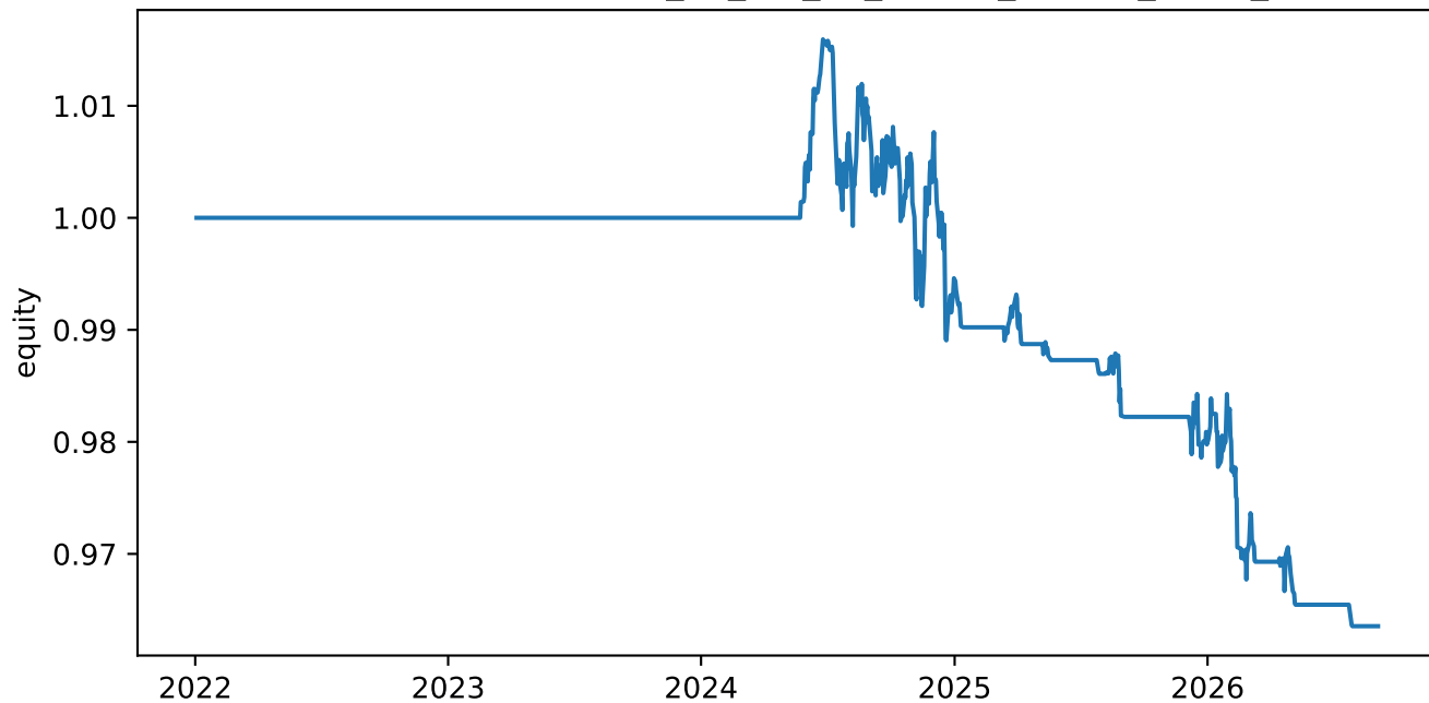
H-005 sealed OOS block_05_flat_10_ols504_adf252_ez1.5_z90
