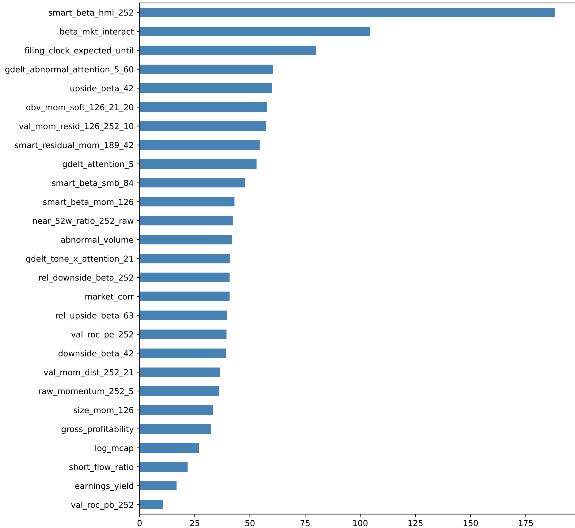
LightGBM feature importance (gain) — IS model; insight only
