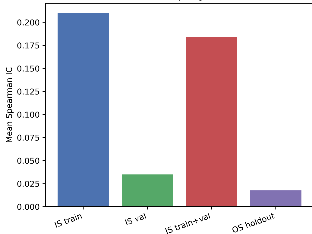
Mean IC by segment
