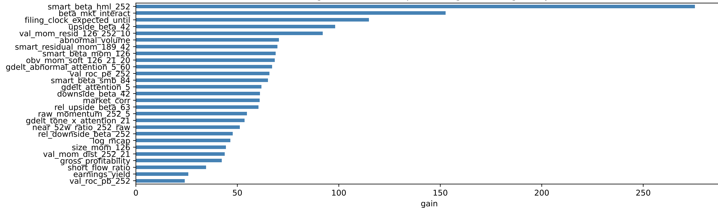
LightGBM feature importance (gain) — insight only
