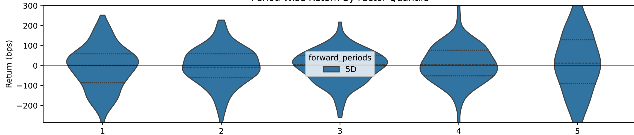
Period Wise Return By Factor Quantile
