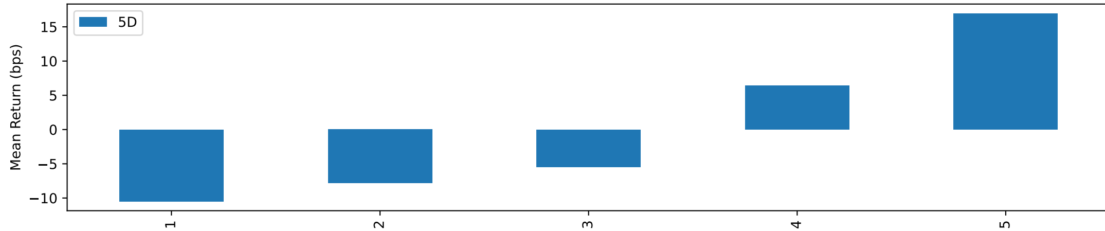
Mean Period Wise Return By Factor Quantile
