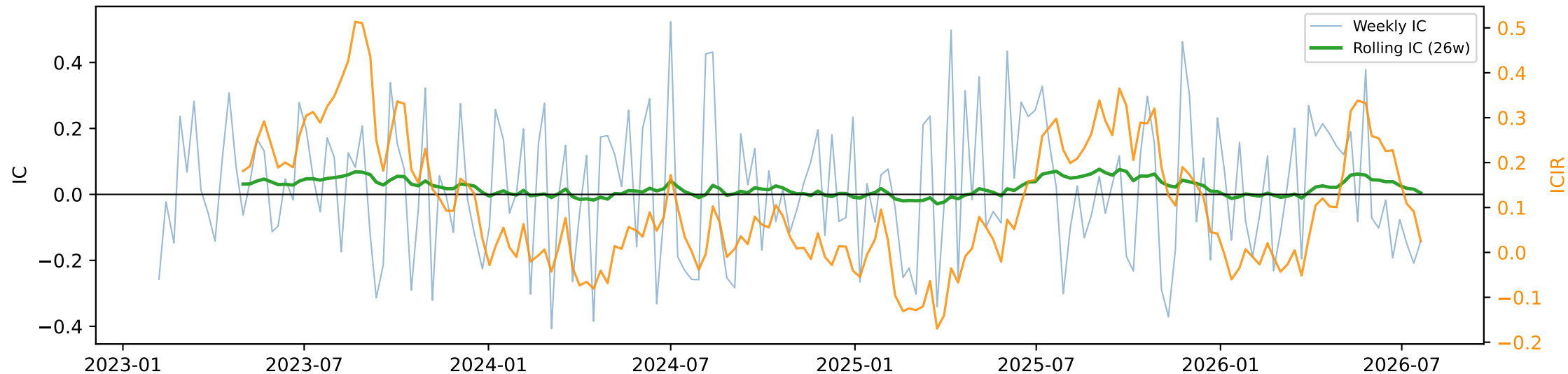
Holdout weekly IC and rolling mean IC
