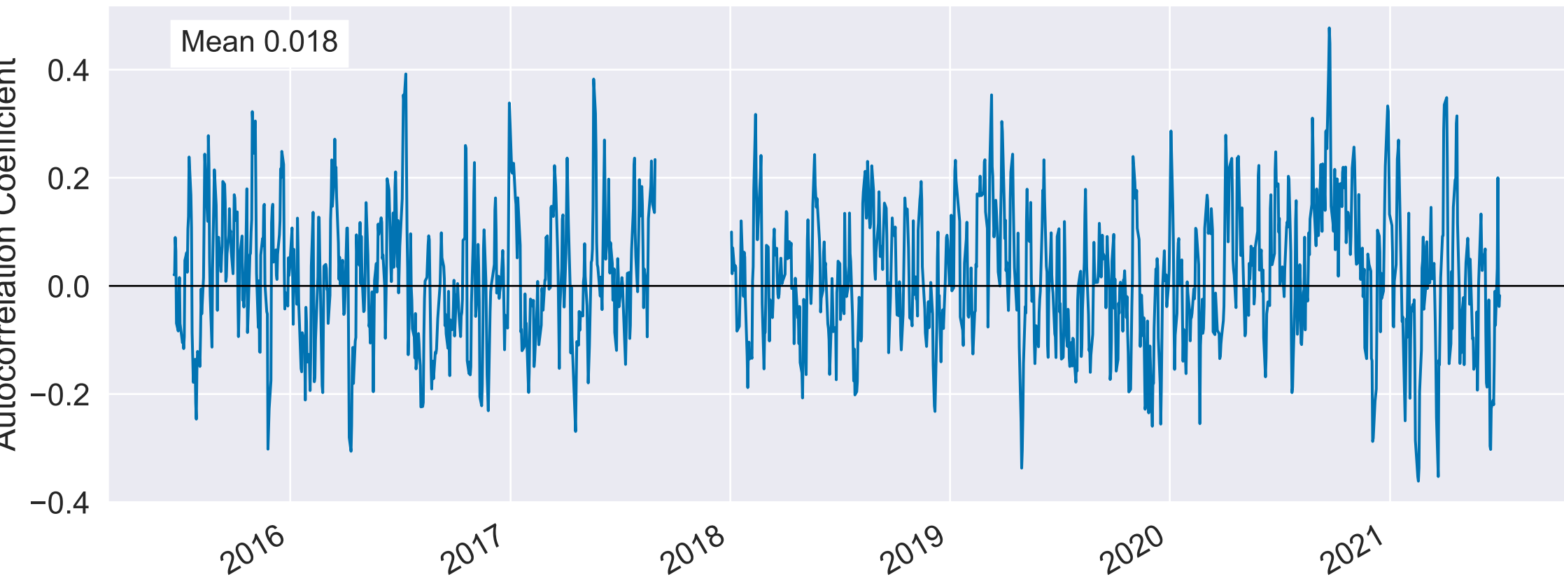
21D Period Factor Rank Autocorrelation
