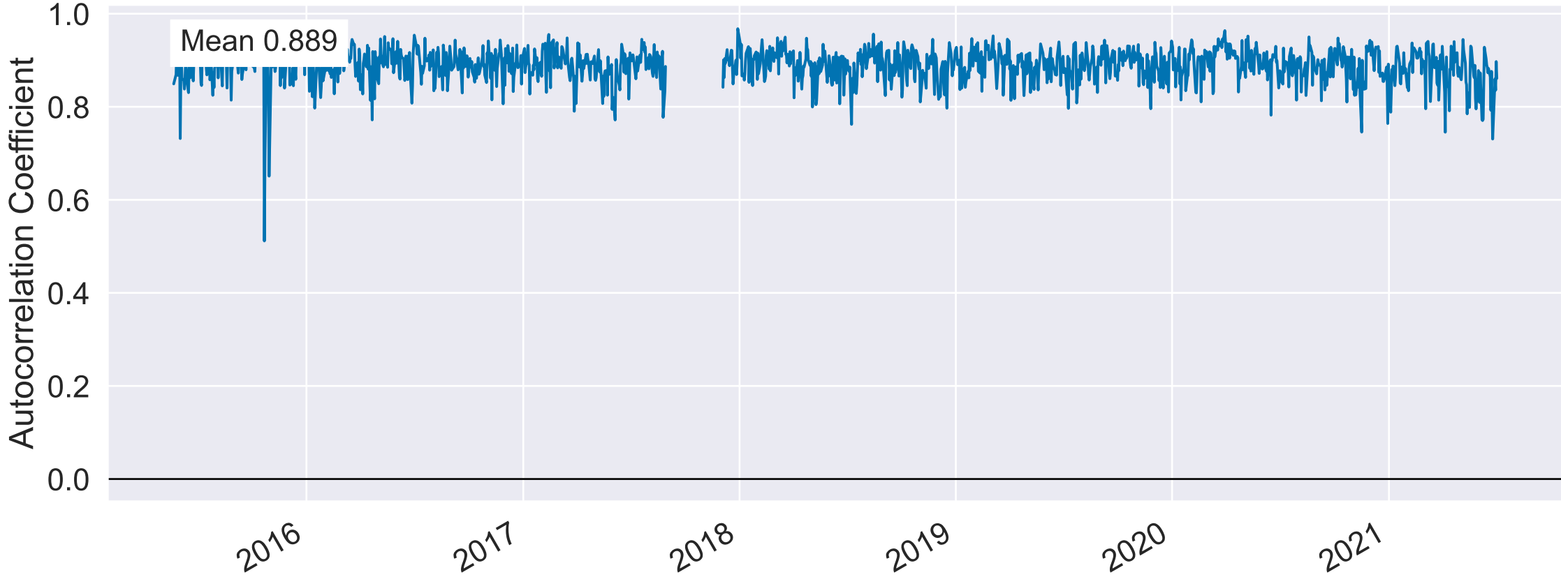
5D Period Factor Rank Autocorrelation
