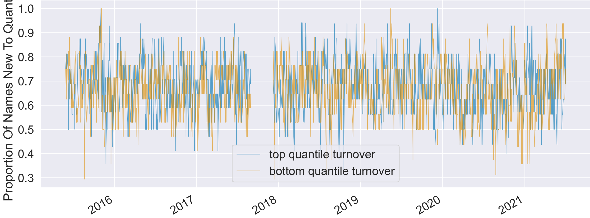
21D Period Top and Bottom Quantile Turnover
