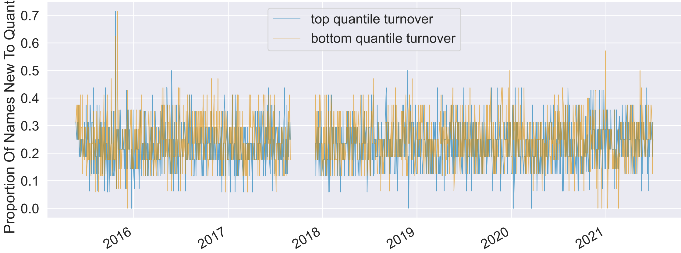
5D Period Top and Bottom Quantile Turnover
