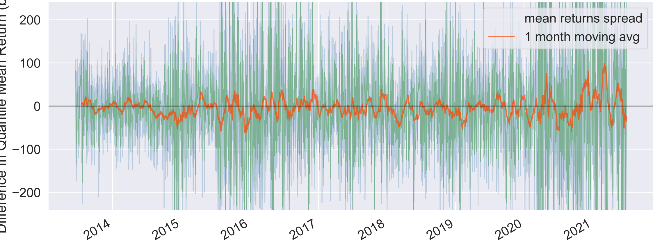
Top Minus Bottom Quantile Mean Return (5D Period Forward Return)
