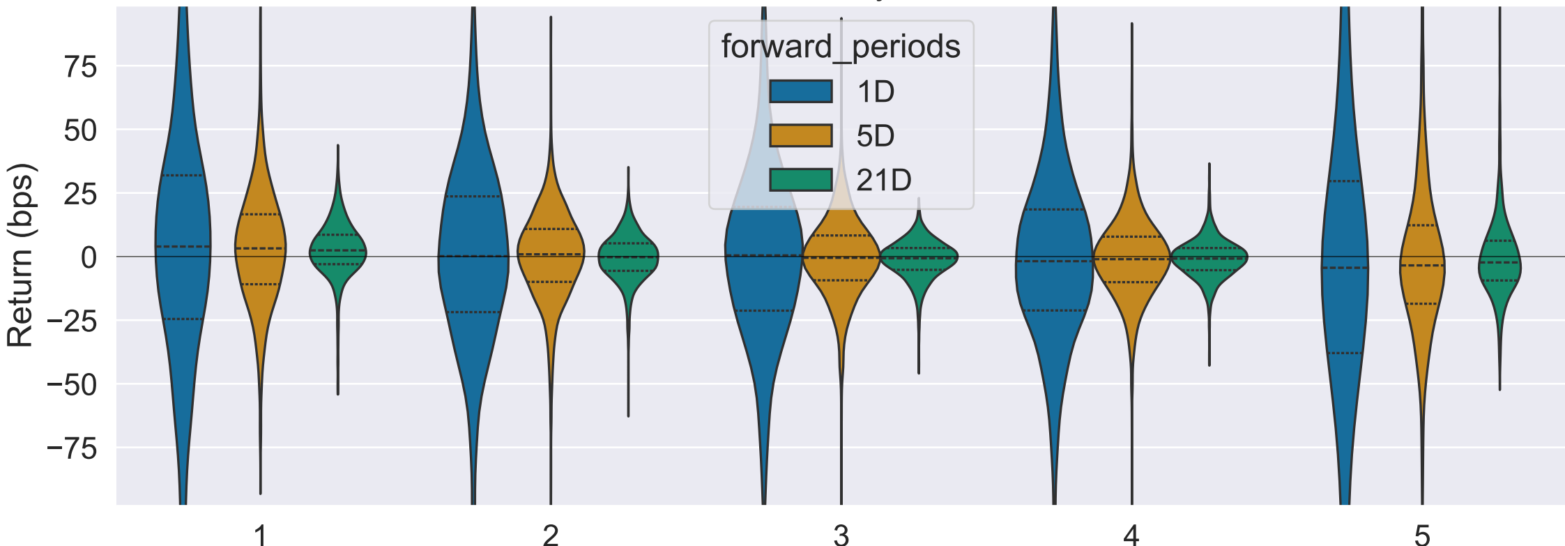
Period Wise Return By Factor Quantile
