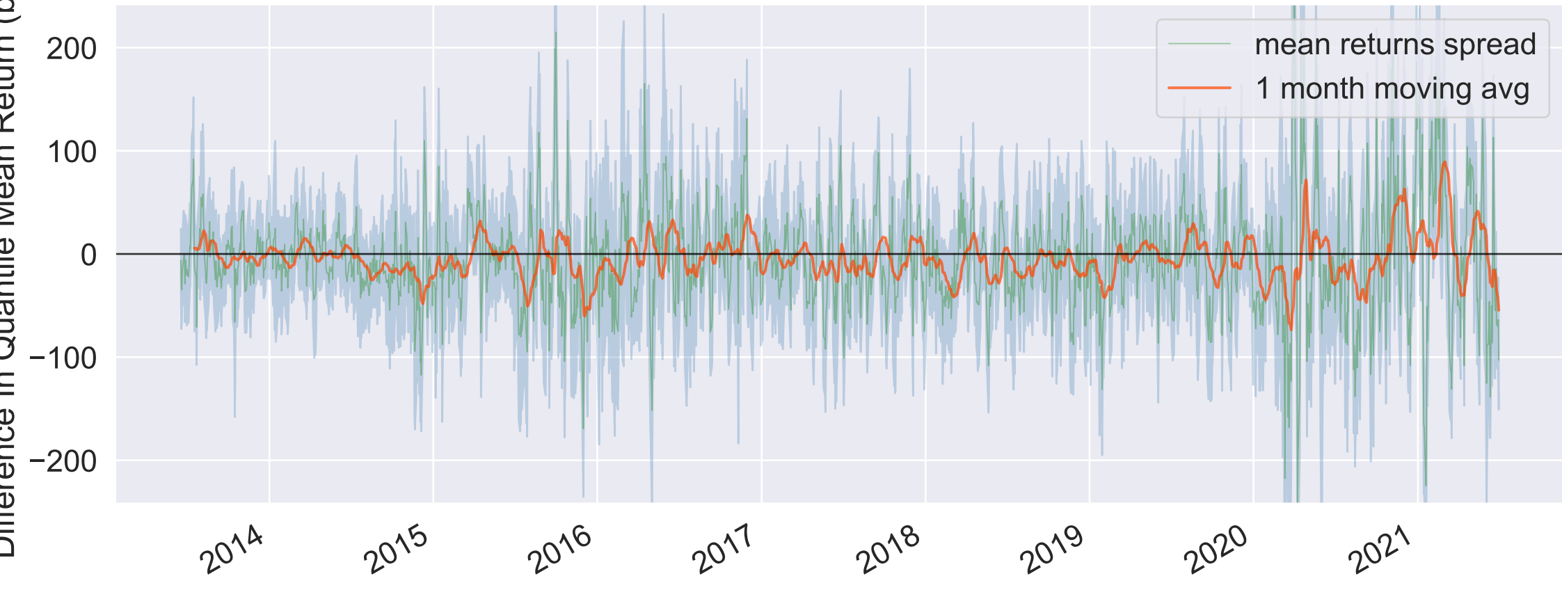
Top Minus Bottom Quantile Mean Return (21D Period Forward Return)
