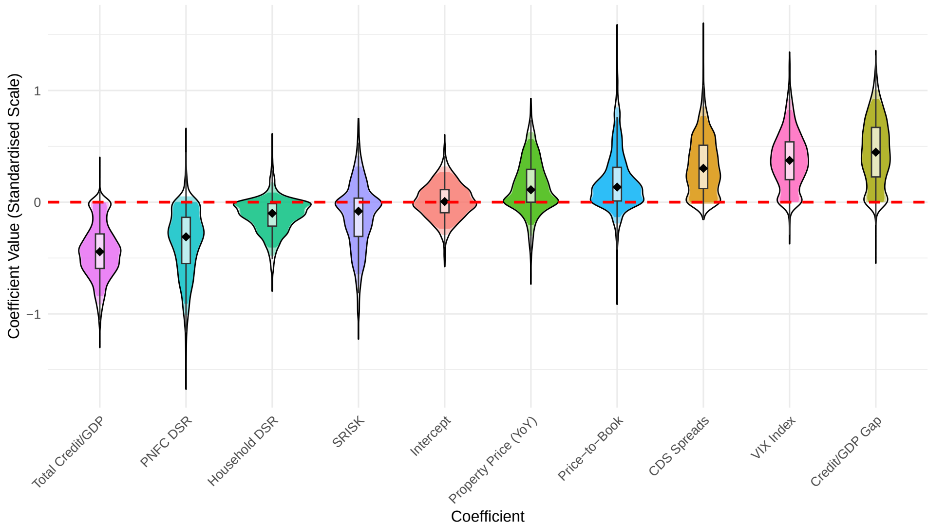
Distribution of Ridge Coefficients (Lagged) (2000 Bootstraps)
