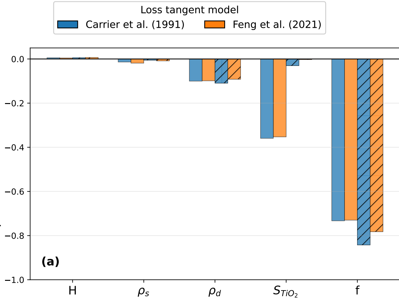
Spearman correlation
