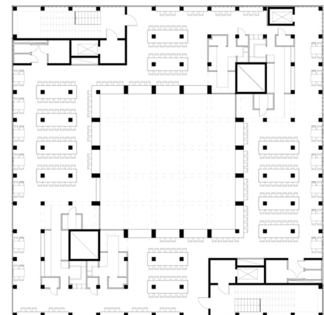
PLAN 1 1:200 (A1)
