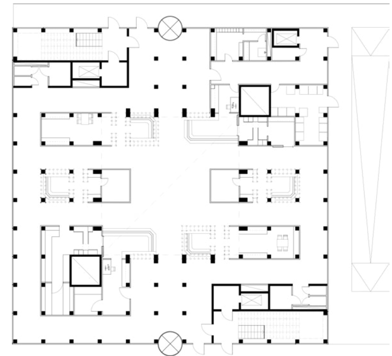
ENTREPLAN 1:200 (A1)
