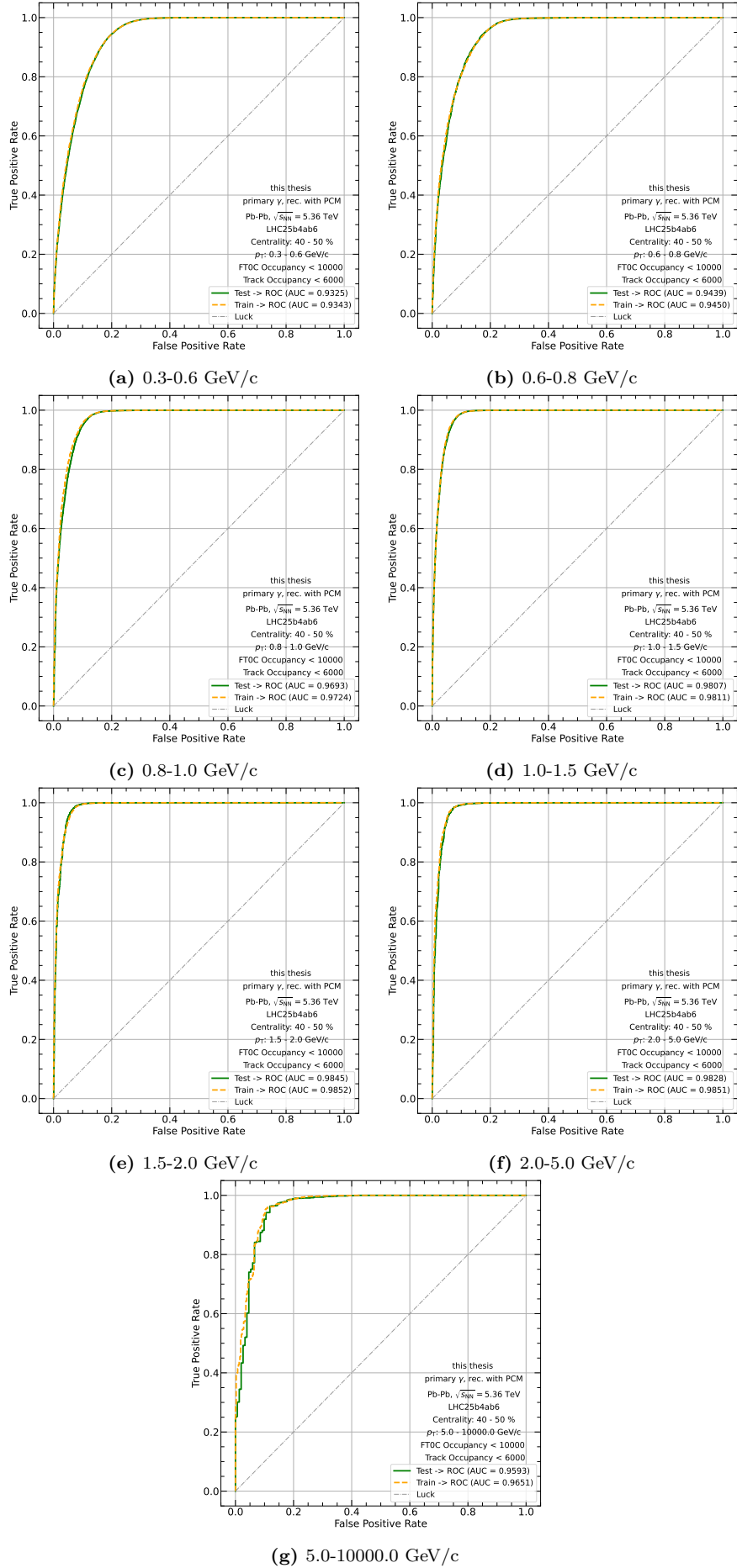
Figure 15: ML model ROC curve with corresponding AUC values for all p_T bins in the centrality range 40-50 %
