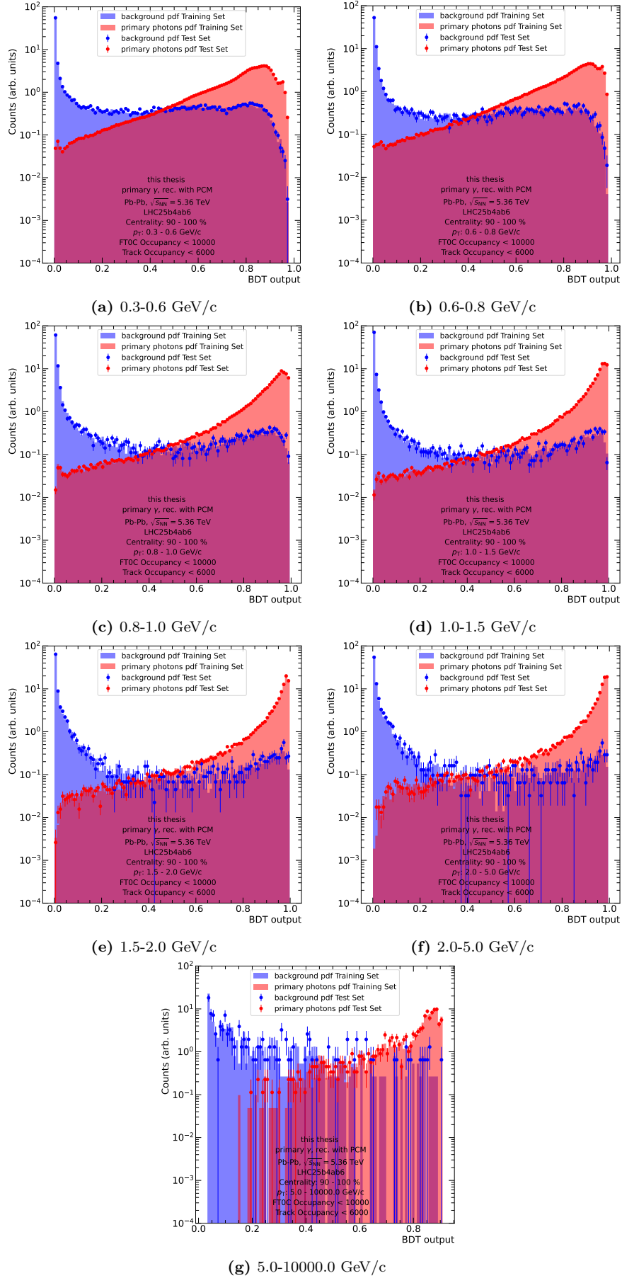
Figure 10: ML model output for all p_T bins in the centrality range 90-100 %
