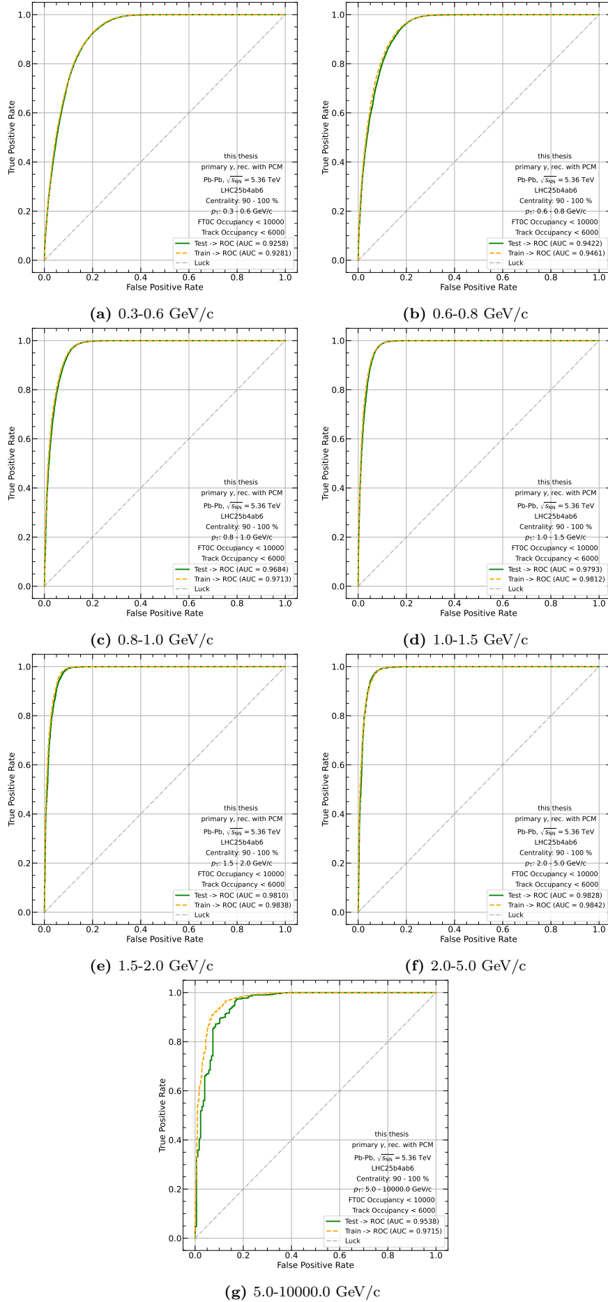
Figure 20: ML model ROC curve with corresponding AUC values for all p_T bins in the centrality range 90-100 %
