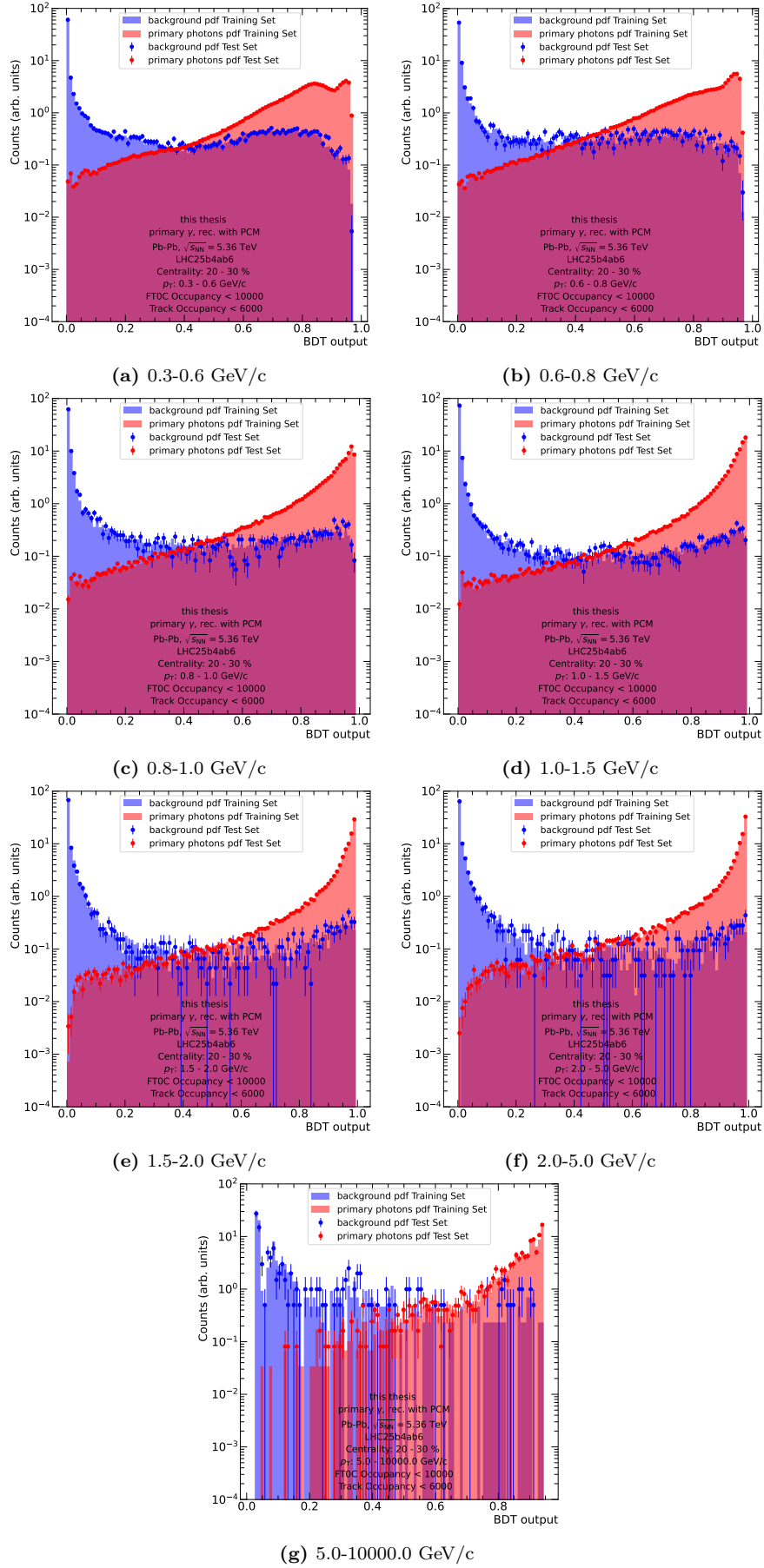
Figure 3: ML model output for all p_T bins in the centrality range 20-30 %
