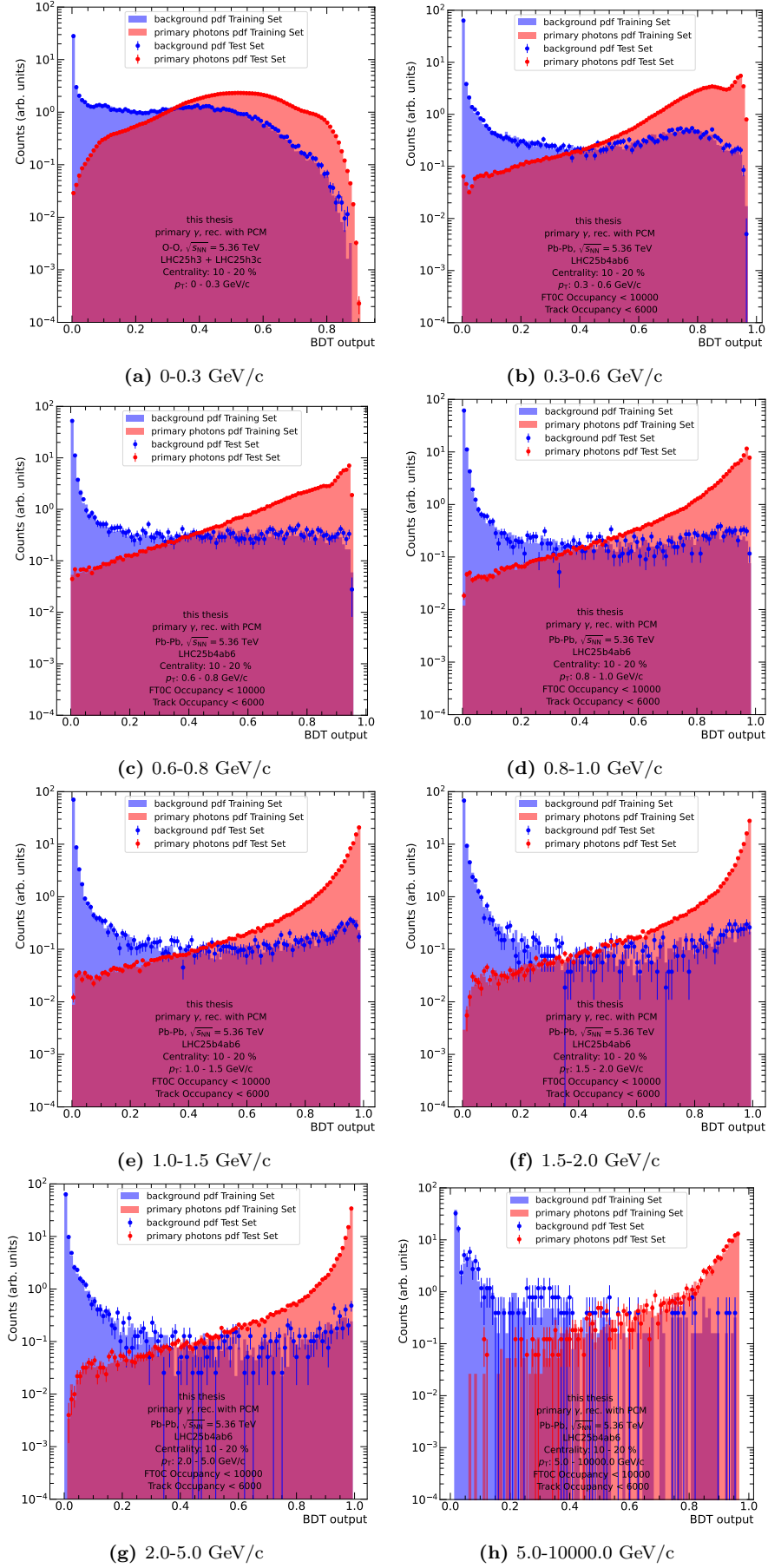
Figure 2: ML model output for all p_T bins in the centrality range 10-20 %
