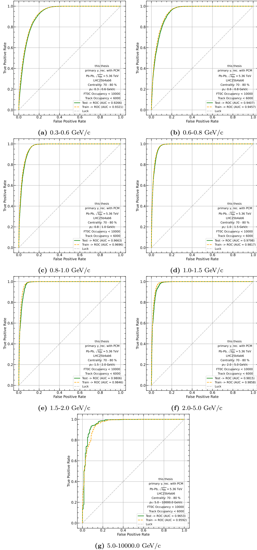
Figure 18: ML model ROC curve with corresponding AUC values for all p_T bins in the centrality range 70-80 %
