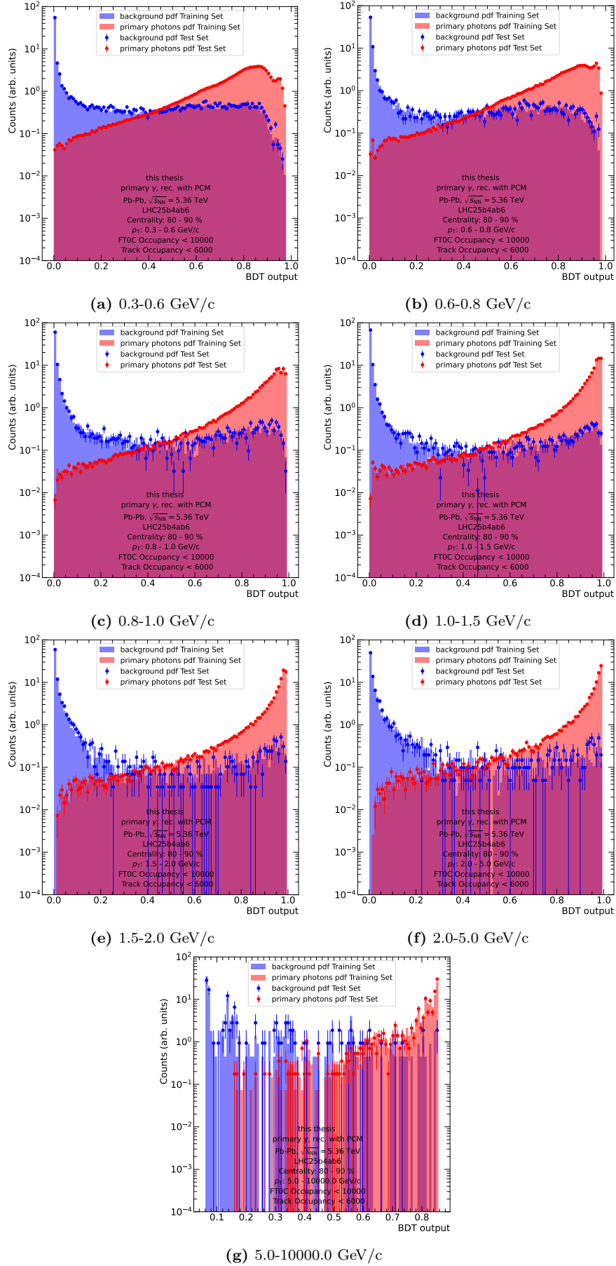
Figure 9: ML model output for all p_T bins in the centrality range 80-90 %
