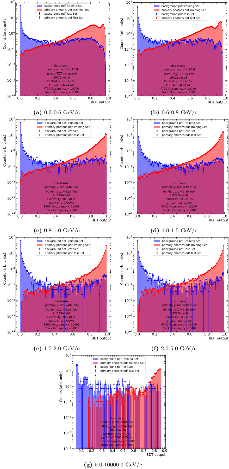
Figure 4: ML model output for all p_T bins in the centrality range 30-40 %
