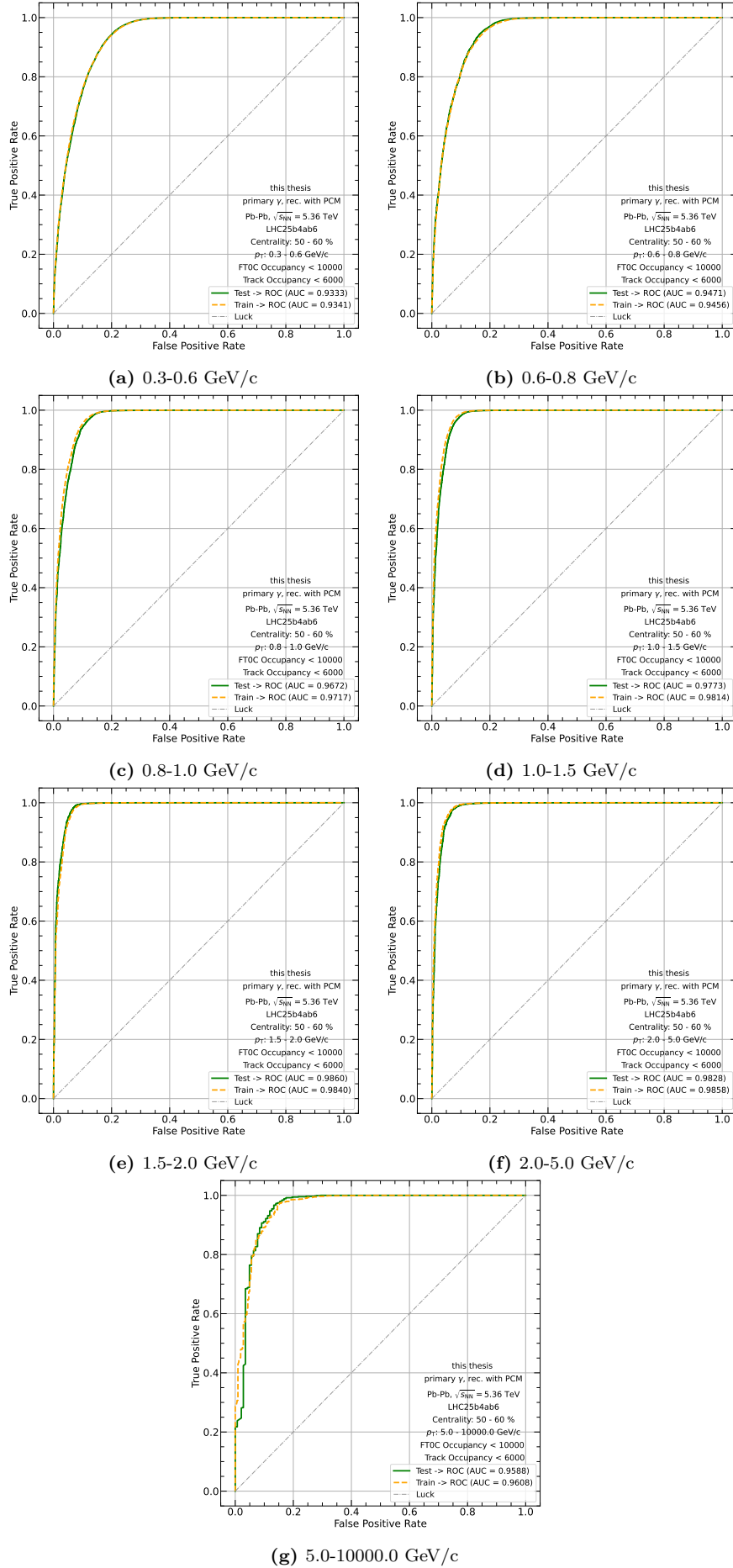
Figure 16: ML model ROC curve with corresponding AUC values for all p_T bins in the centrality range 50-60 %
