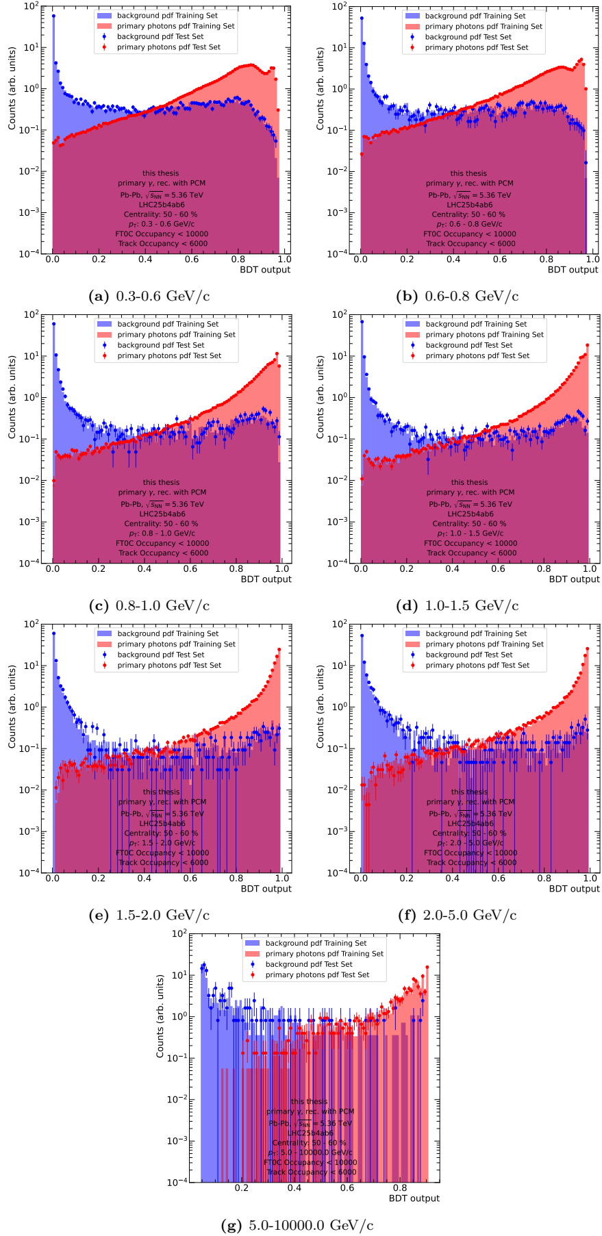
Figure 6: ML model output for all p_T bins in the centrality range 50-60 %
