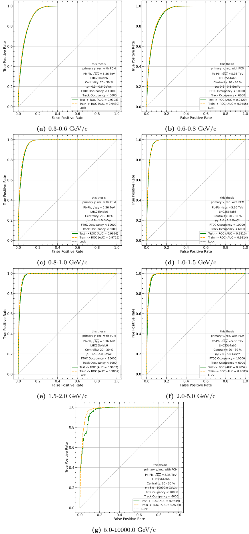
Figure 13: ML model ROC curve with corresponding AUC values for all p_T bins in the centrality range 20-30 %
