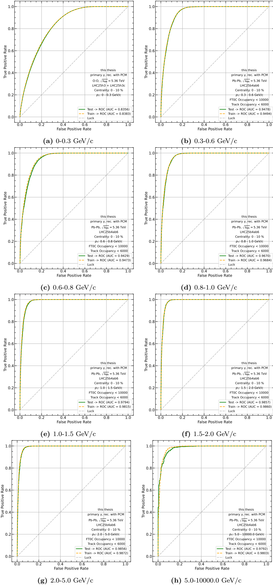
Figure 11: ML model ROC curve with corresponding AUC values for all p_T bins in the centrality range 0-10 %
