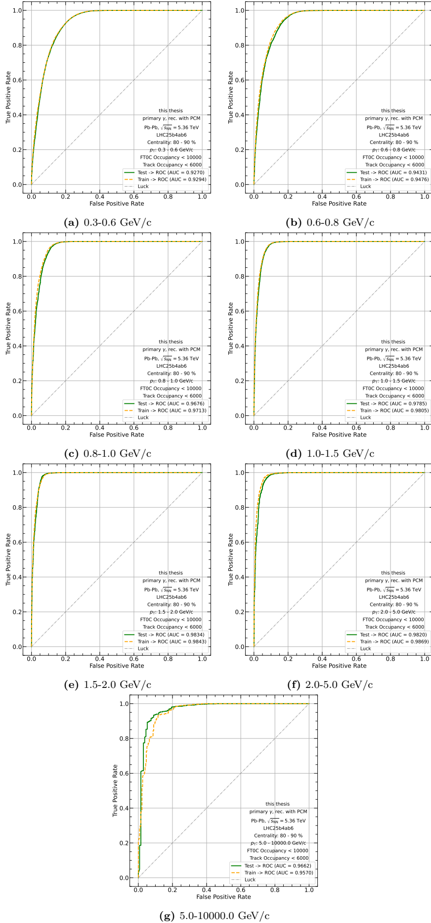
Figure 19: ML model ROC curve with corresponding AUC values for all p_T bins in the centrality range 80-90 %
