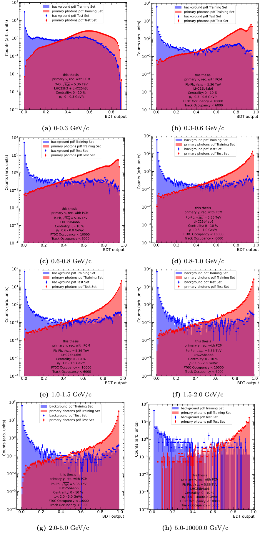
Figure 1: ML model output for all p_T bins in the centrality range 0-10 %
