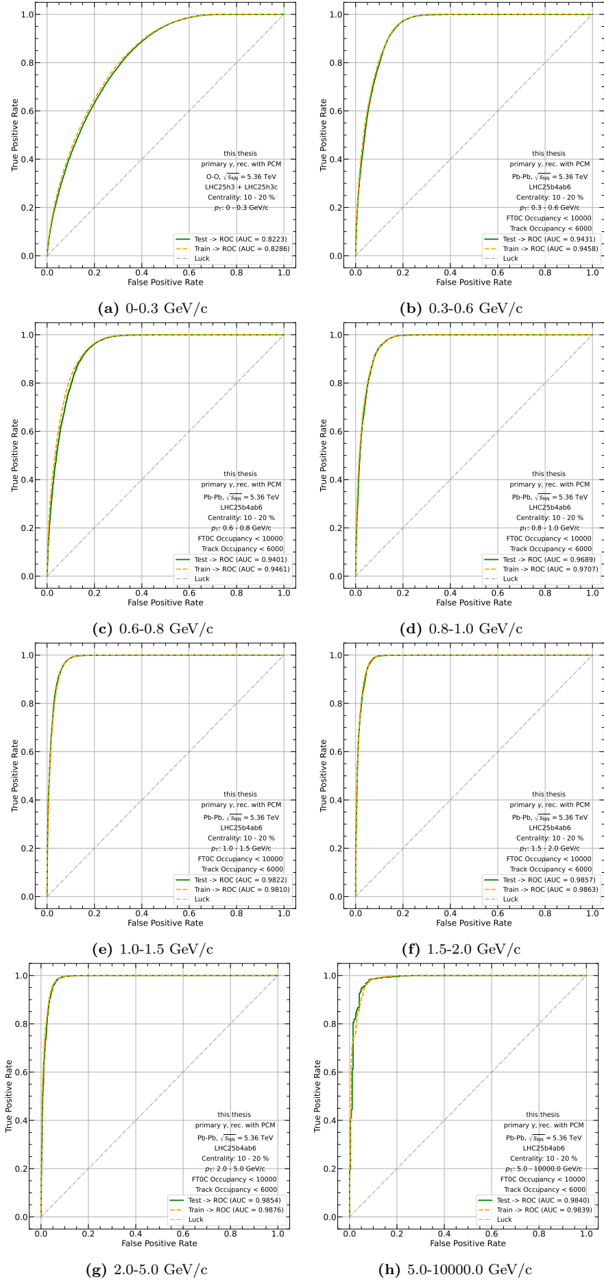
Figure 12: ML model ROC curve with corresponding AUC values for all p_T bins in the centrality range 10-20 %
