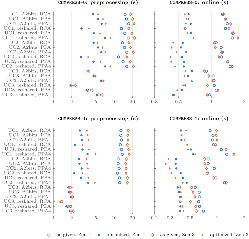
Figure 16: The 36 all_opt builds on ImageNet (dummy weights) by use case, as given and optimized, on both machine pairs (log scale; median of two runs, UC3 of five interleaved runs).
