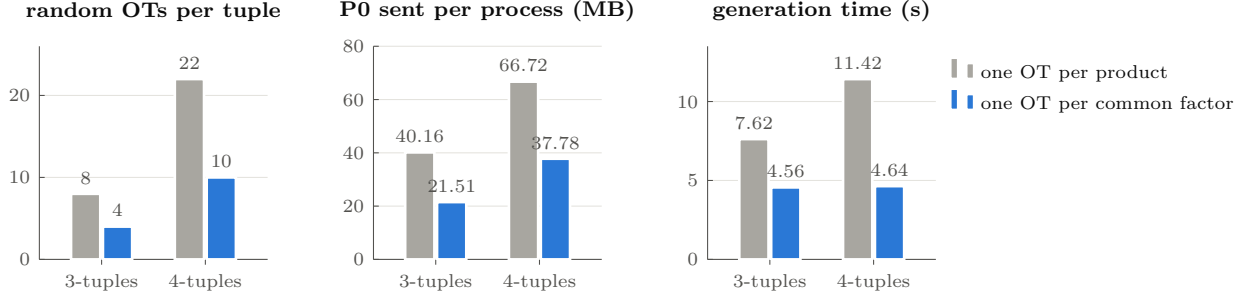
Figure 9: Beaver tuple generation per process in a multi-batch PPA4 run (flare / polynize, 24 processes).
