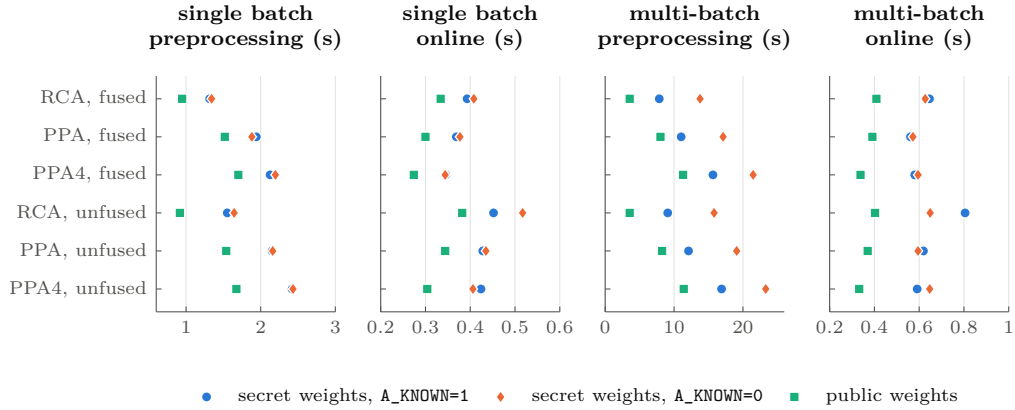
Figure 12: Secret weights with A\_KNOWN=1 (default) and A\_KNOWN=0 , and public weights, plain family, flare / polynize (final builds; multi-batch A\_KNOWN=0 and public weights before the lane batching, which does not apply to them).
