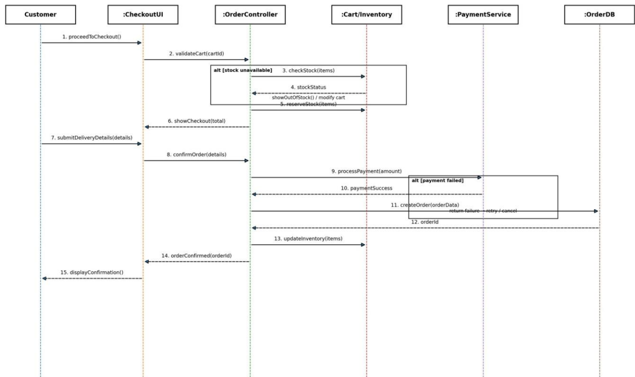
Figure 1: Sequence Diagram - Place an Online Order
