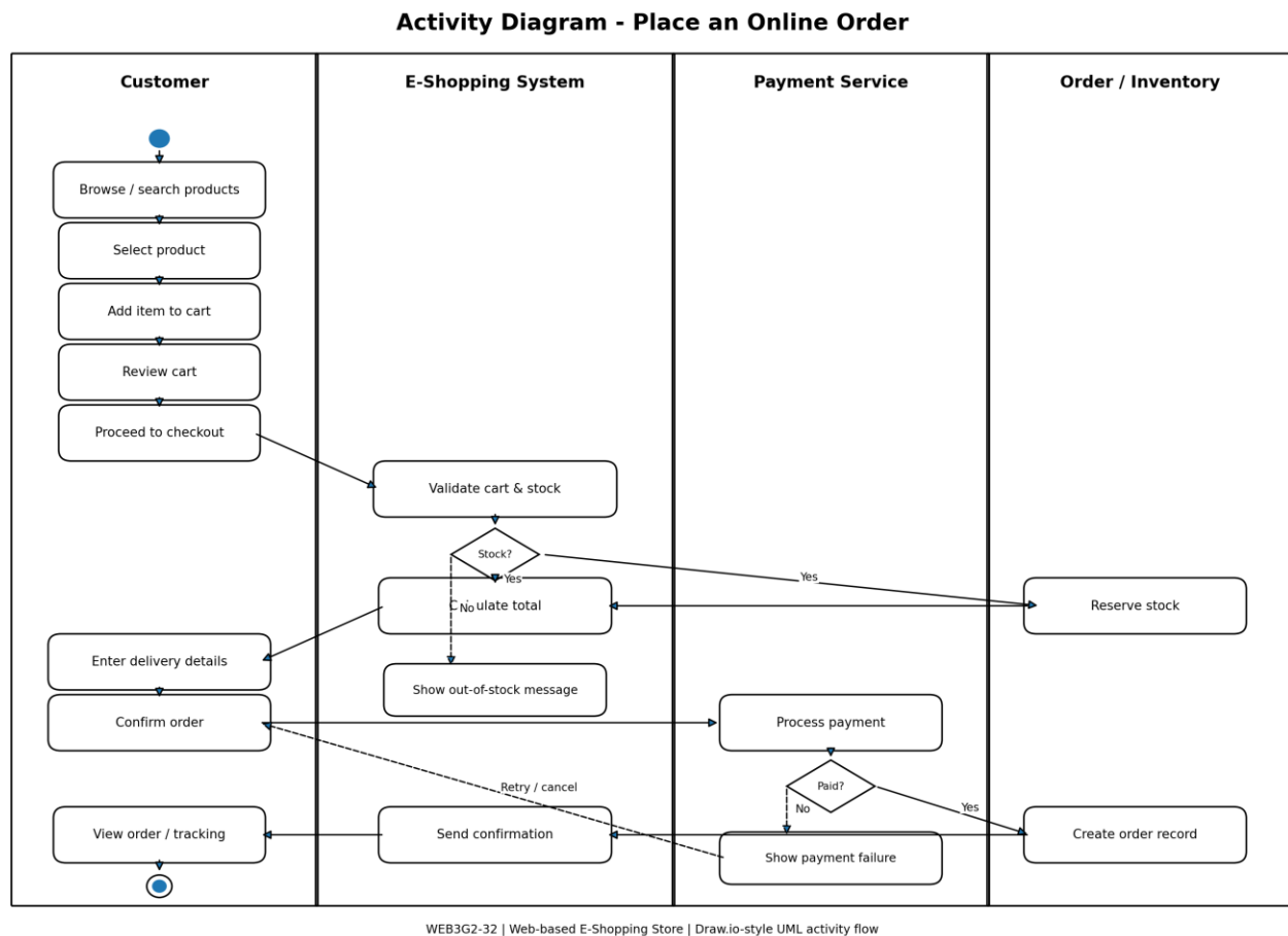
Figure 1: Activity Diagram - Place an Online Order (with swimlanes)
