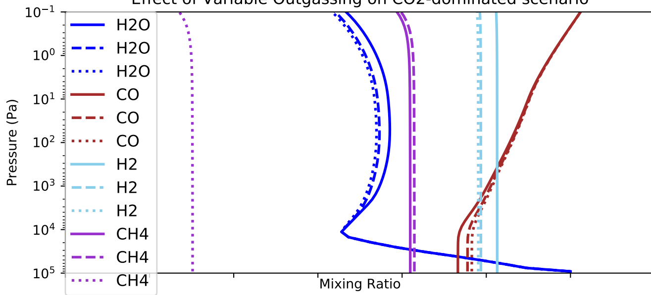
Effect of Variable Outgassing on CO 2 -dominated scenario
