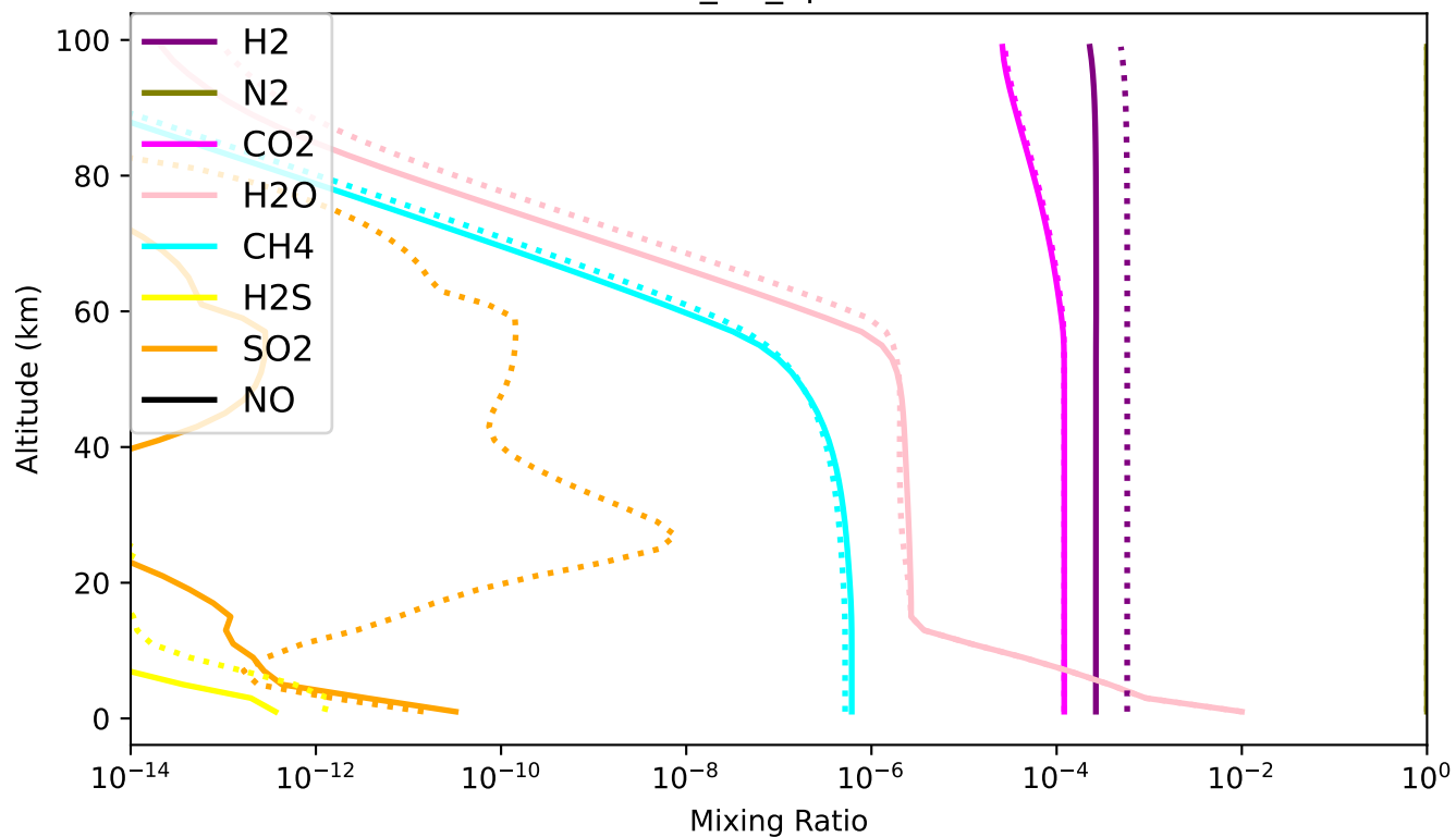
Sun_N2_updates
