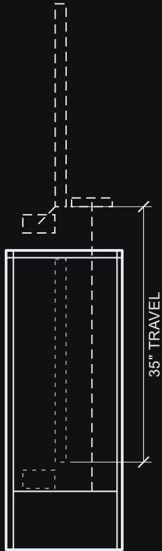
SIDE — SECTION
