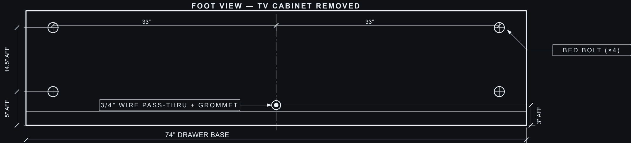
FOOT FACE — MOUNTING PATTERN
