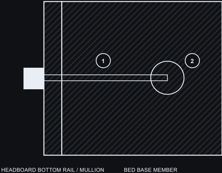
DETAIL — BED-BOLT CONNECTION (HEADBOARD TO BASE)
