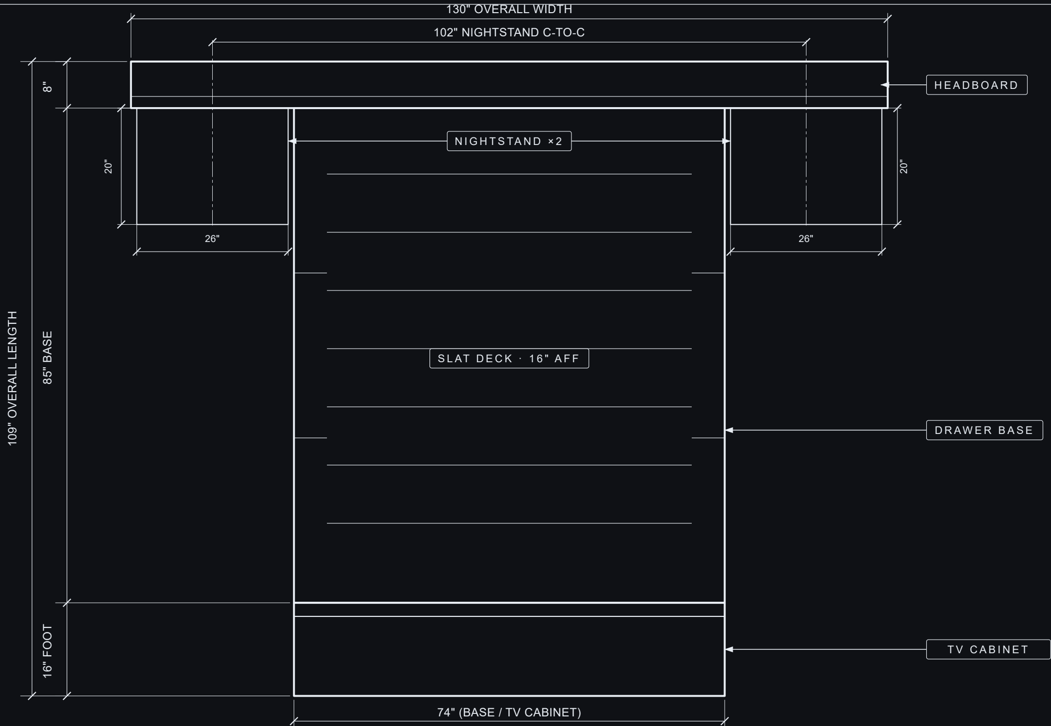
TOP VIEW
