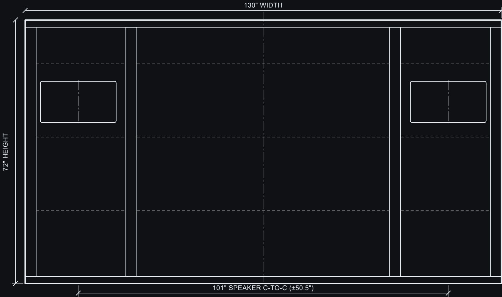
FRONT VIEW
