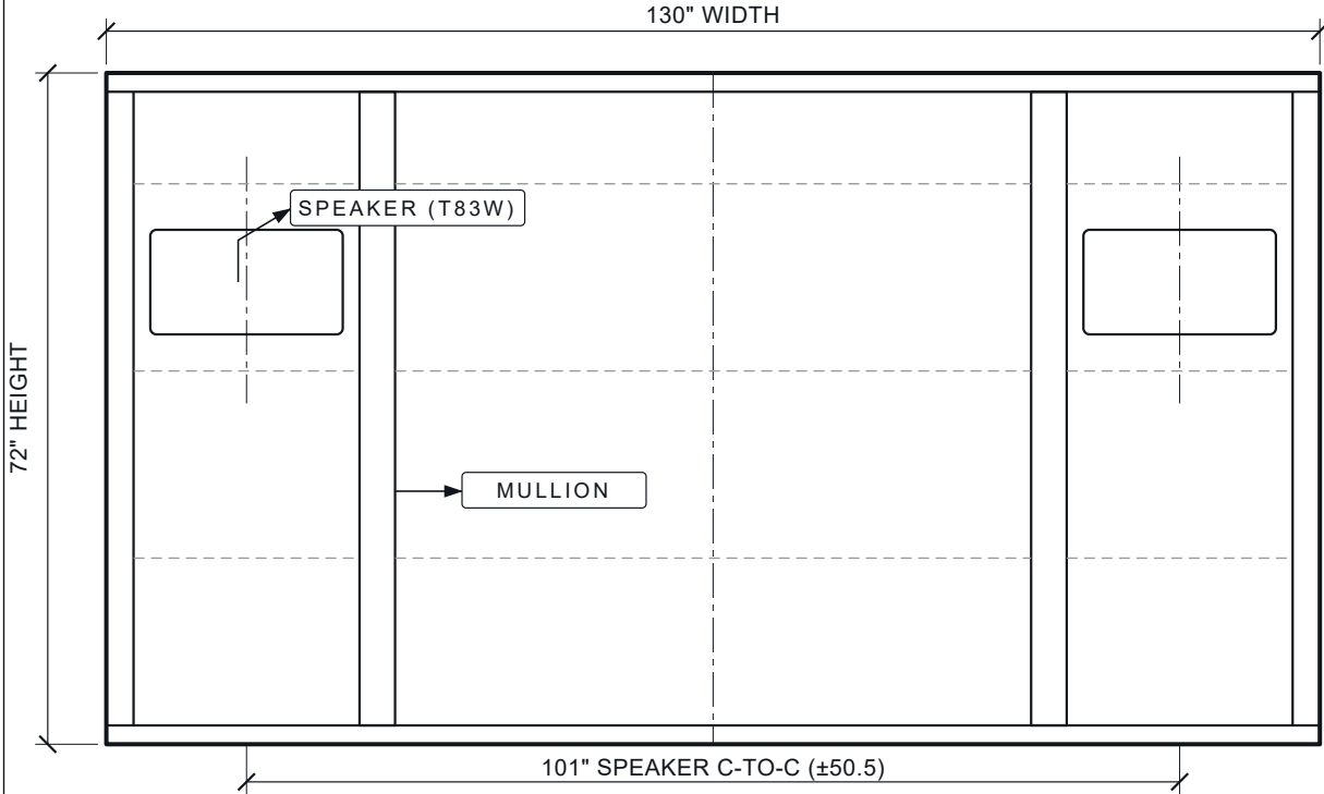
FRONT ELEVATION
