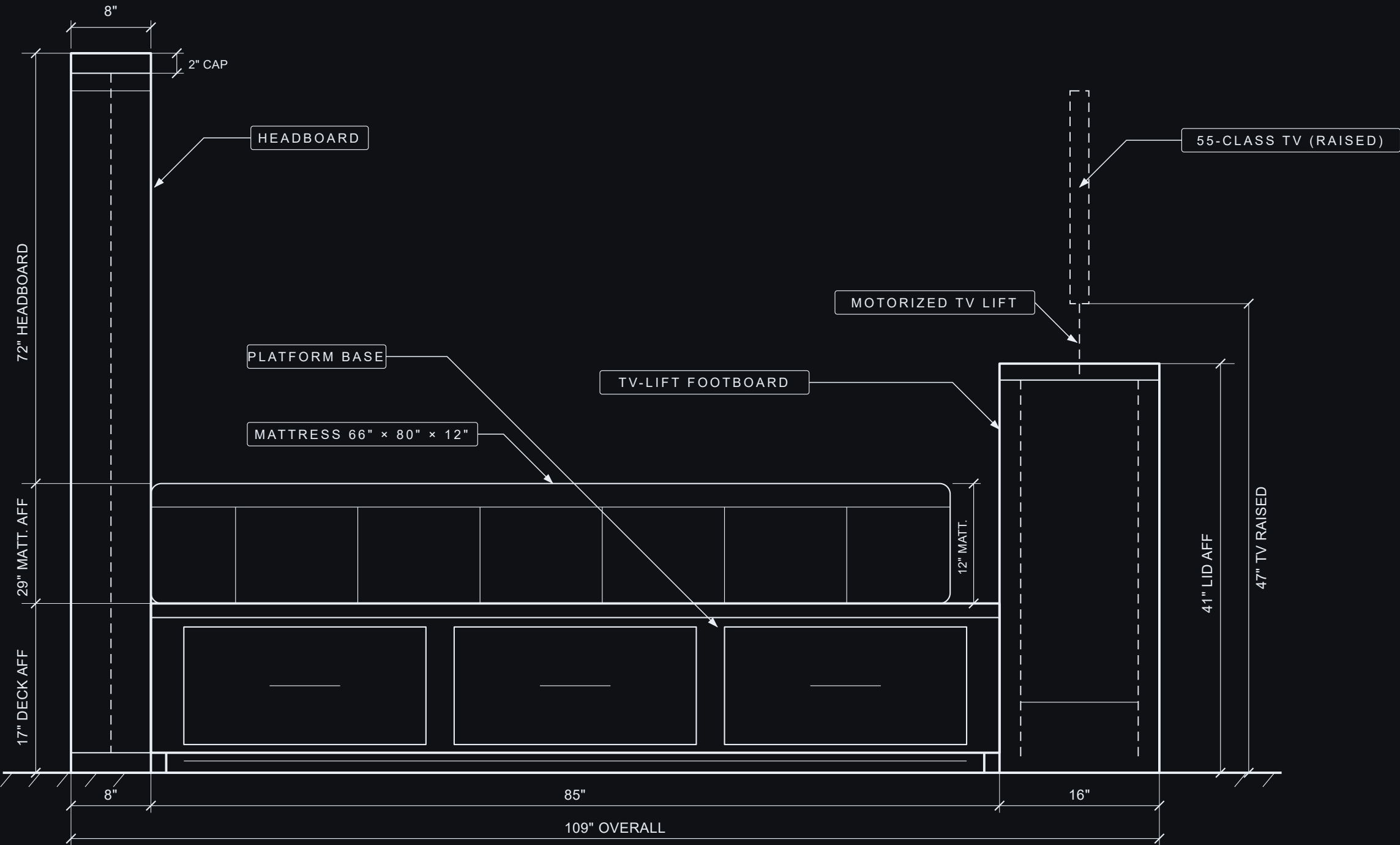
SIDE VIEW
