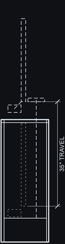
SIDE — SECTION
