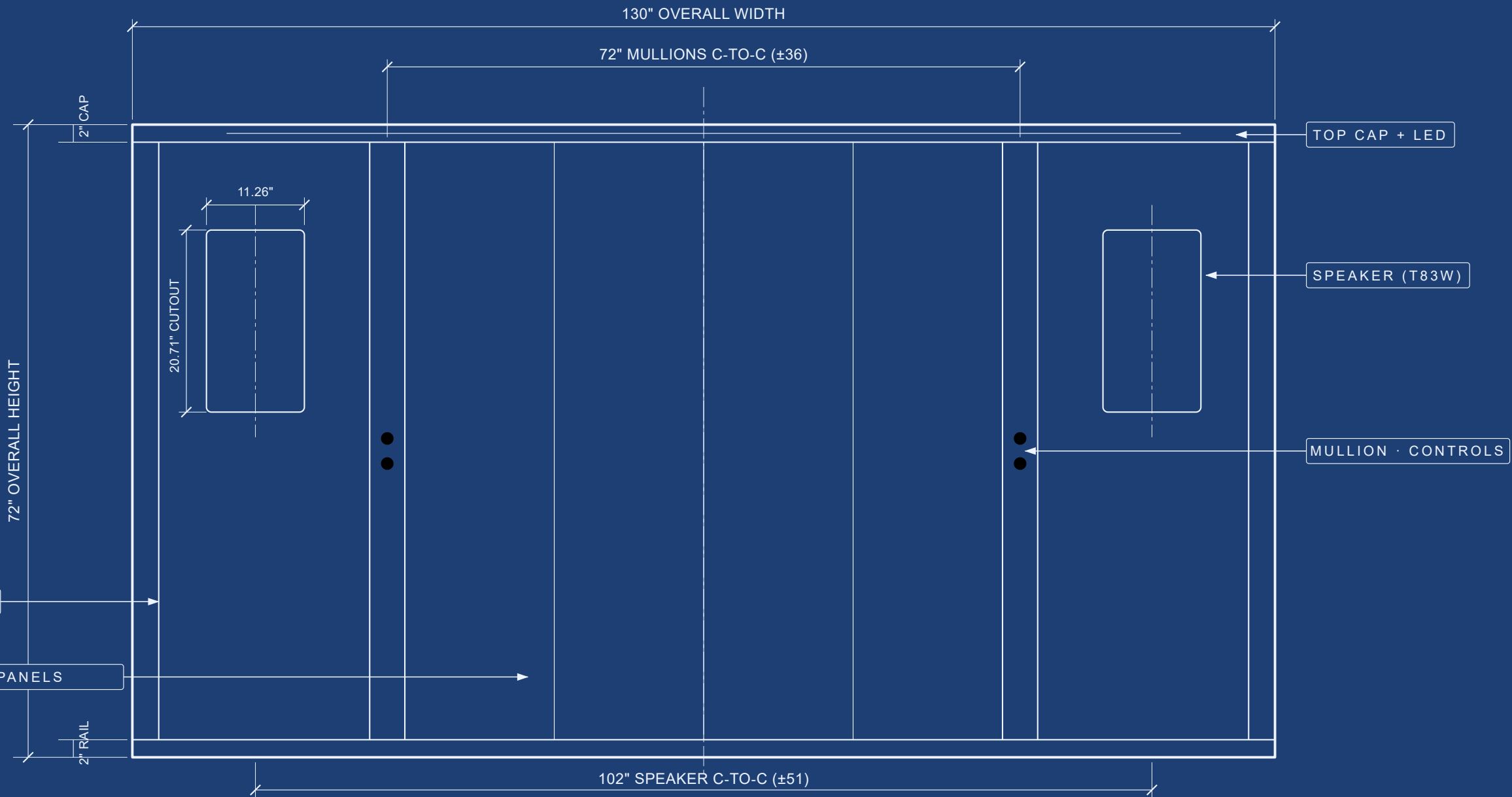
HEADBOARD — FRONT ELEVATION
