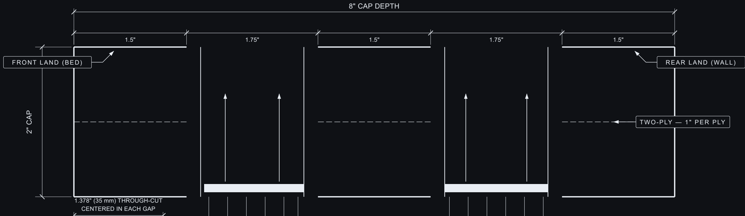
TOP-CAP LED CHANNEL — SECTION
