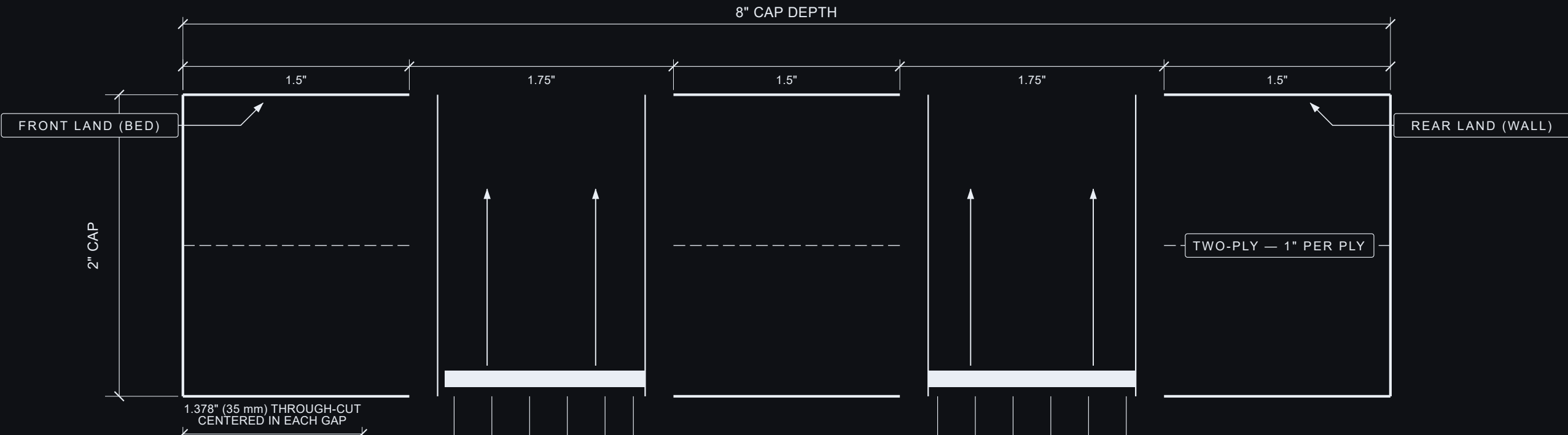
TOP-CAP LED CHANNEL — SECTION
