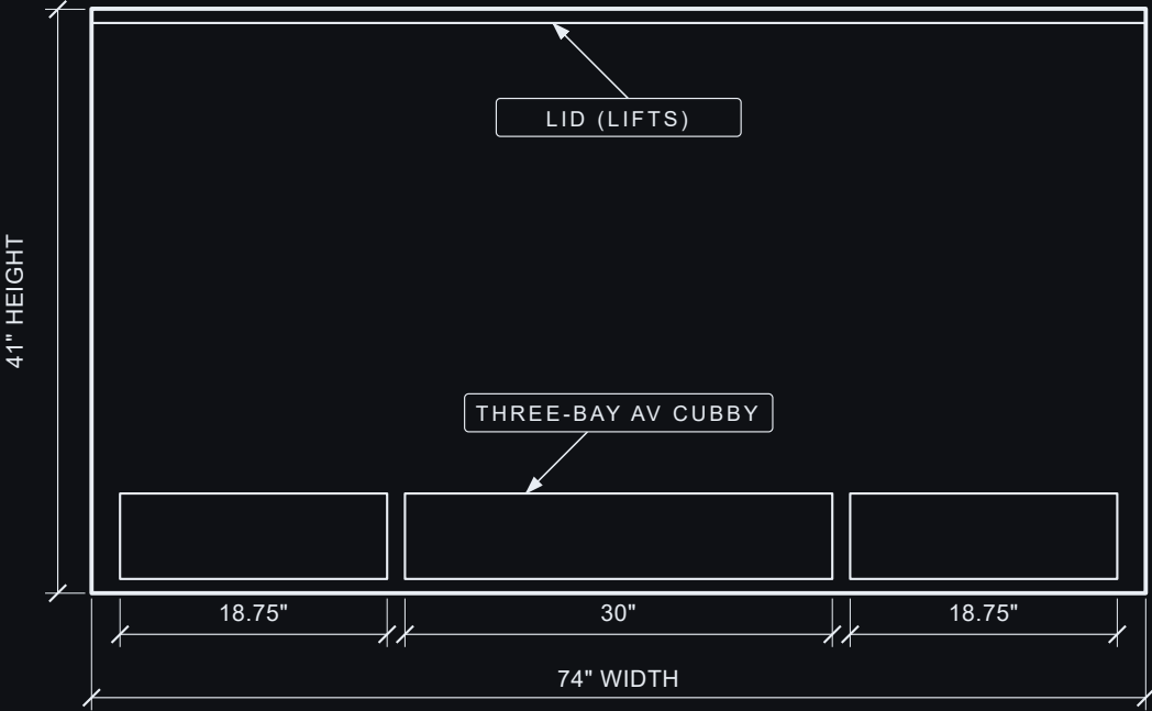
FRONT VIEW
