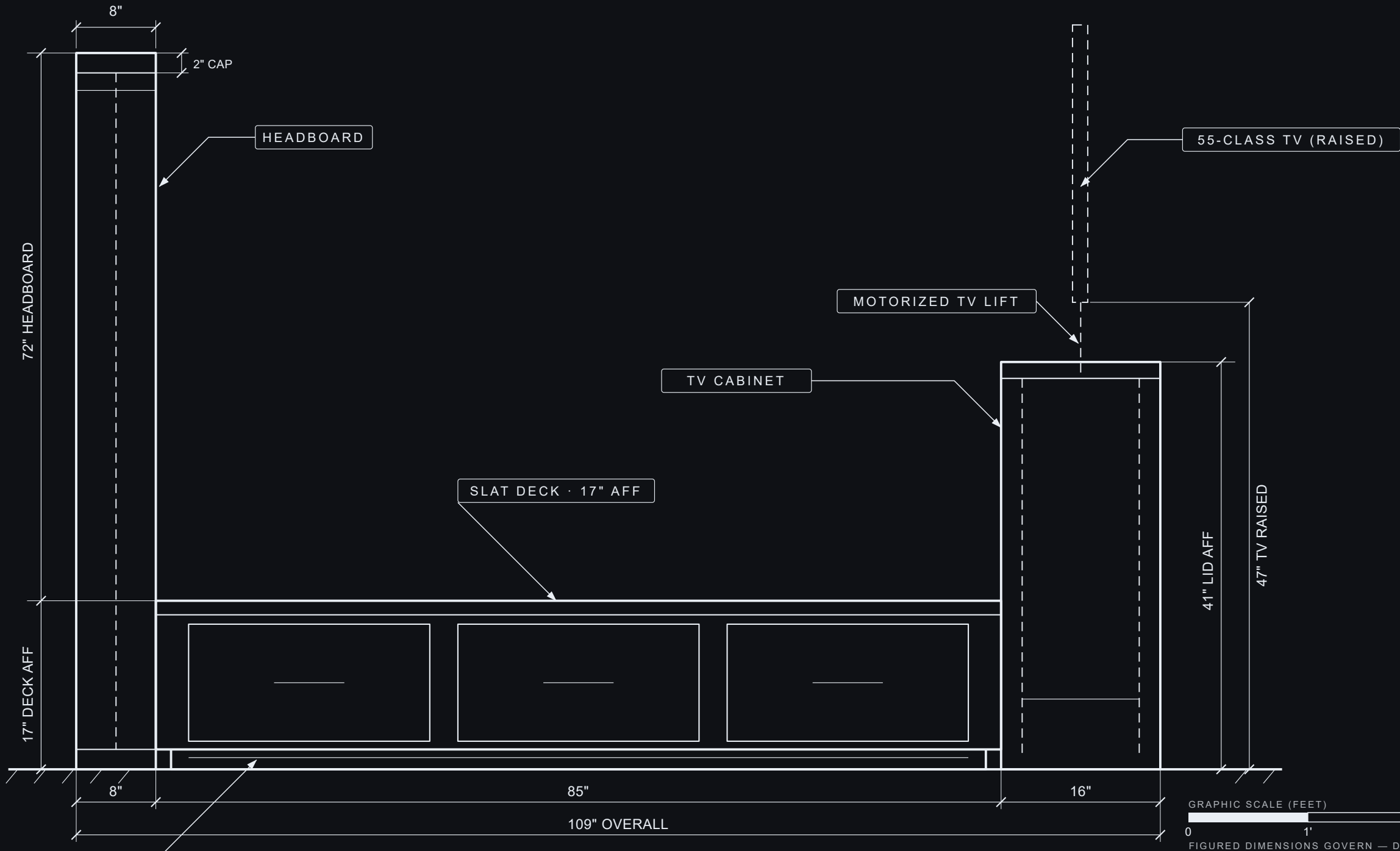
SIDE VIEW
