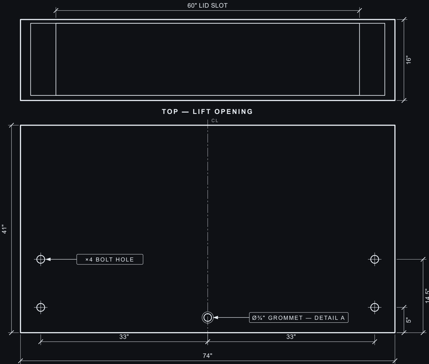
BED-SIDE FACE — BOLTS TO THE BED BASE
