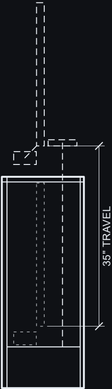
SIDE — SECTION
