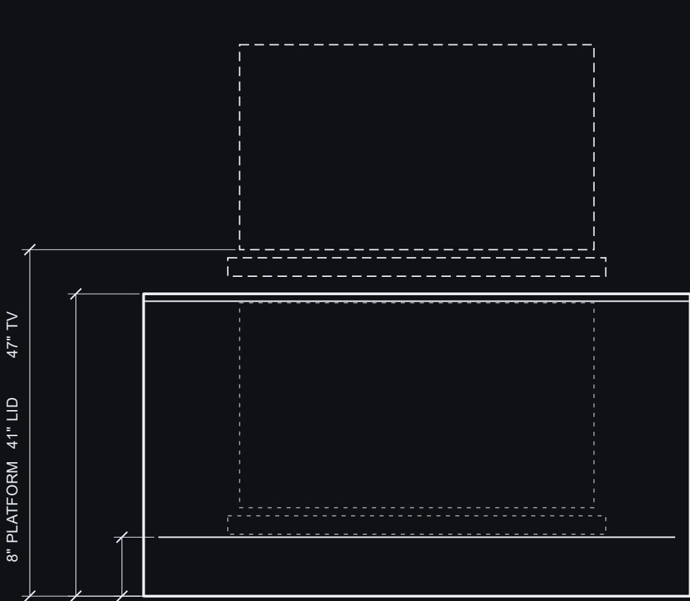
FRONT — TV RAISED
