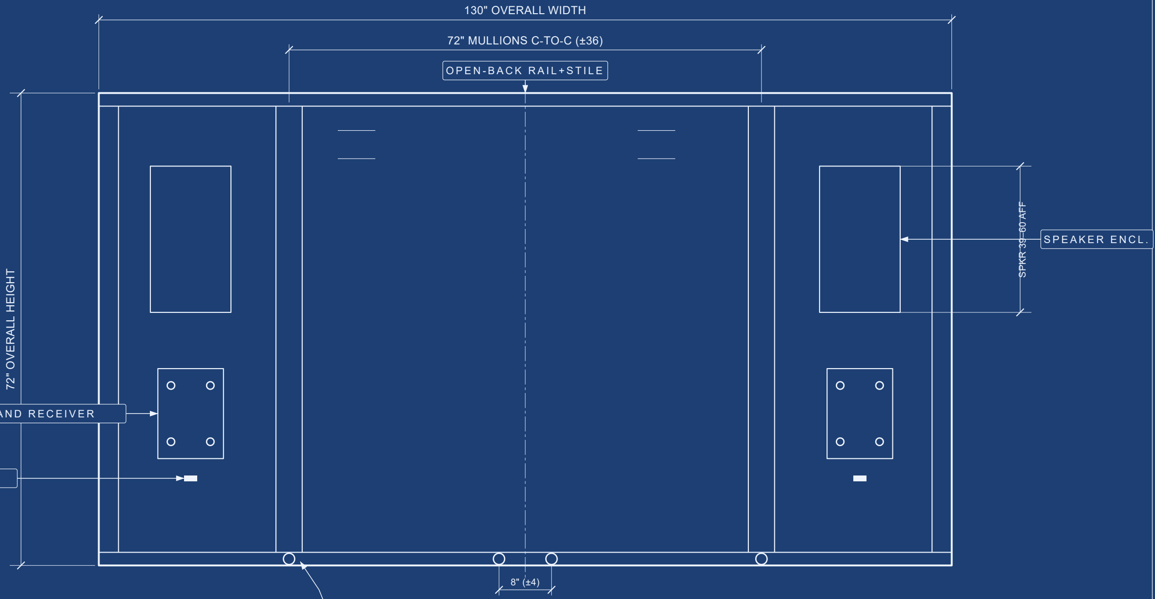
HEADBOARD — REAR ELEVATION
