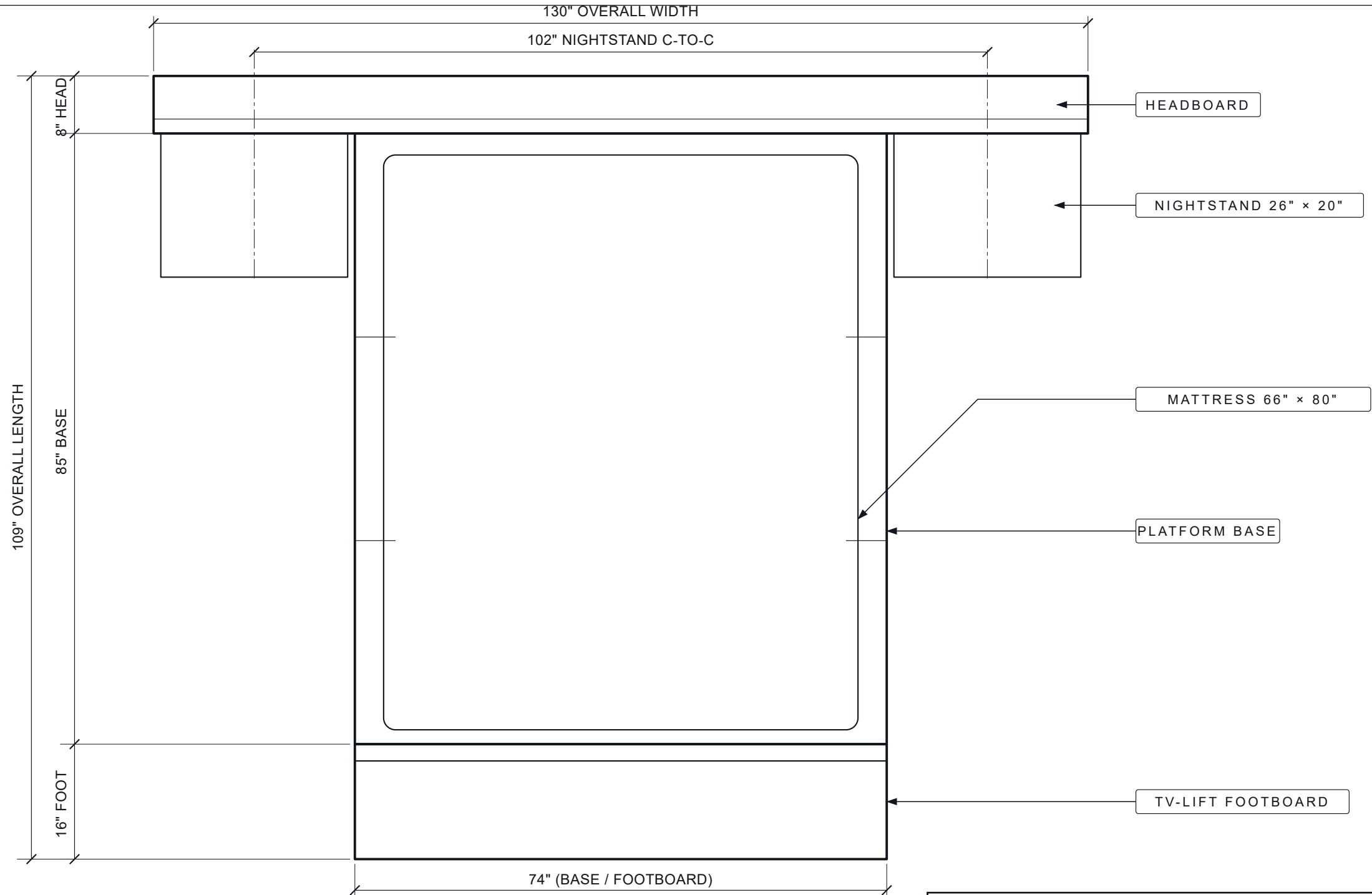
PLAN — TOP DOWN
