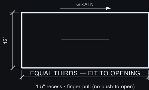
5 DRAWER FACE 1" THK · ×6
