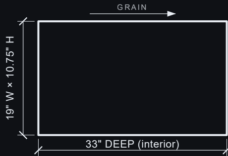
4 DRAWER BOX ×6
