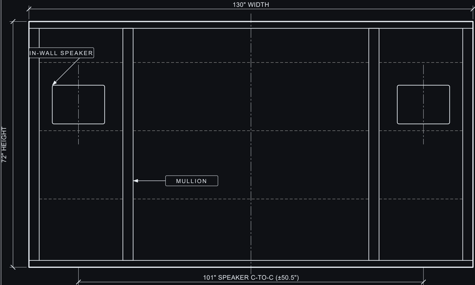
FRONT VIEW
