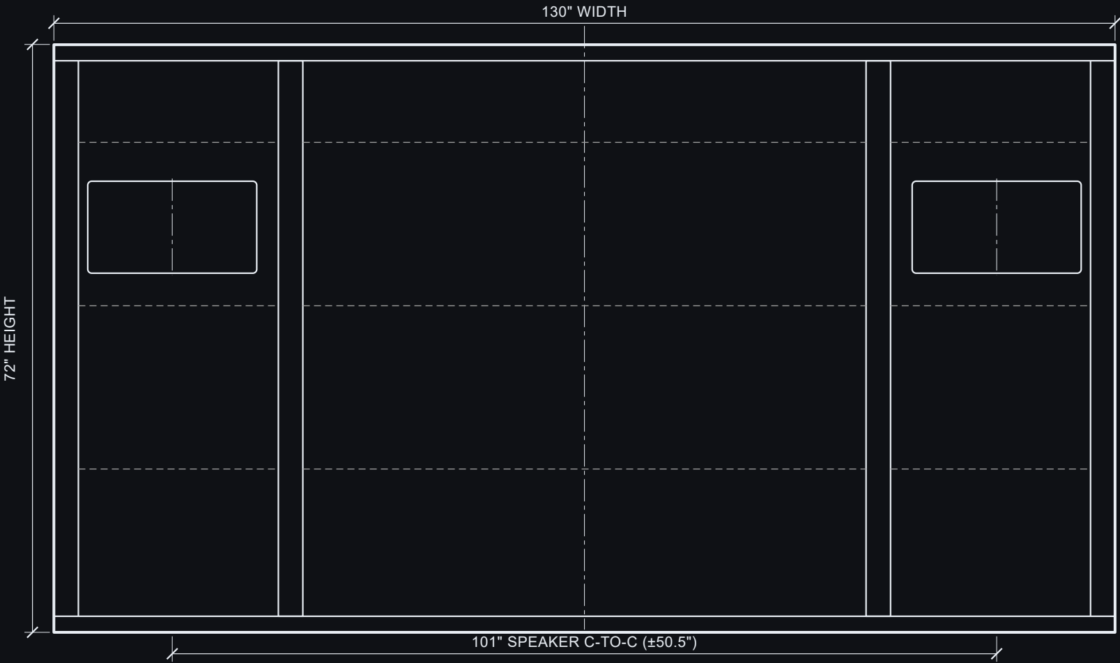
FRONT VIEW
