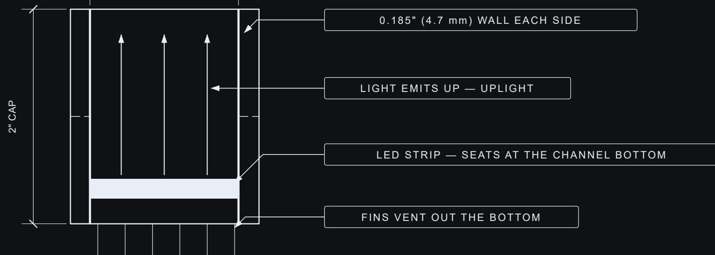
TOP-CAP LED CHANNEL — SECTION
