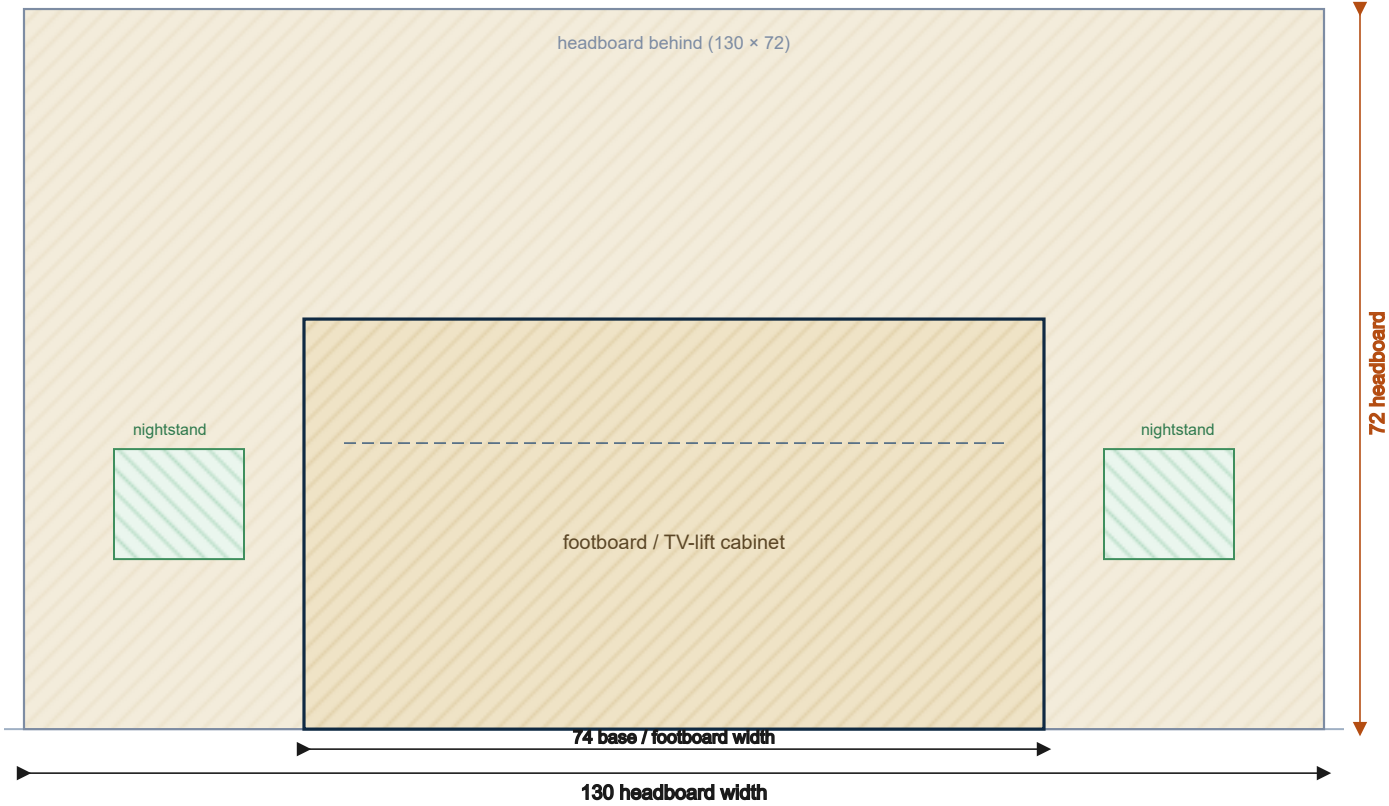
2 · FOOT-END ELEVATION (looking toward the headboard · 1 in = 5 px)
