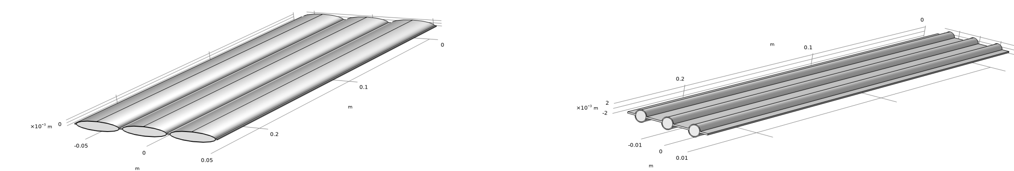
Fig. 2 — Optimal geometry found via Pareto Frontier (left) and the nearly-optimal circular pipe geometry (right), the latter of which is more feasible.
