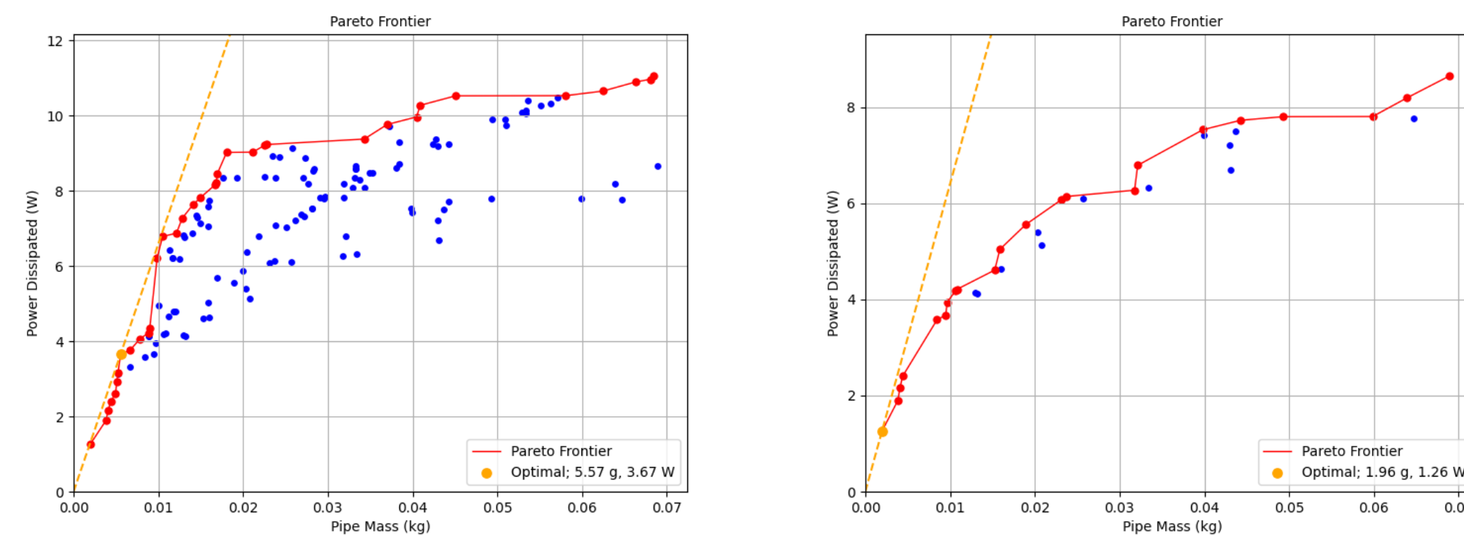
Fig. 1 — Pareto Frontiers showing data from all randomized runs of the simulation (left) and only runs of perfectly circular geometry (right).
