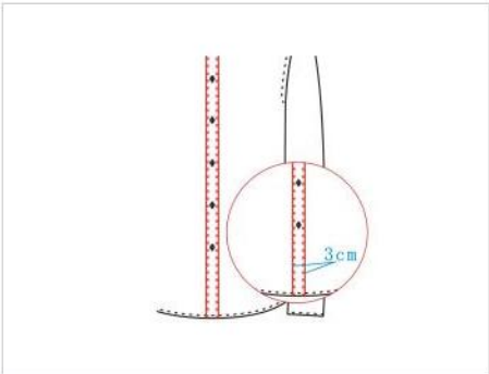
Shirt — 3.0 cm pw-30 Placket Width
