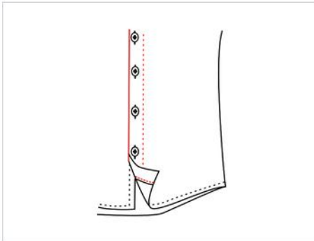
Shirt — Machine 0.1 cm Top Stitching stitch-01-top Placket Decoration Stitching
