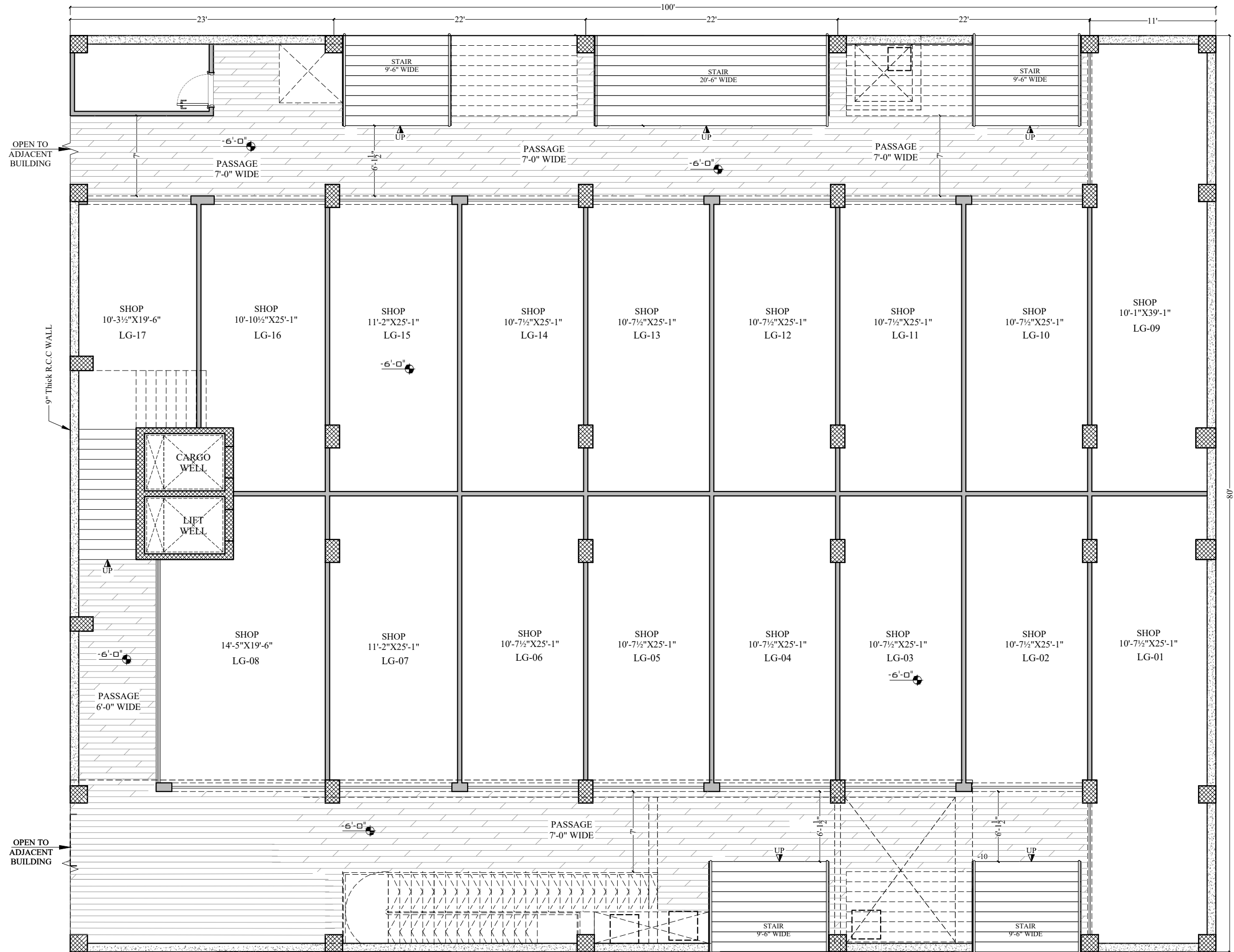
LOWER GROUND FLOOR PLAN
