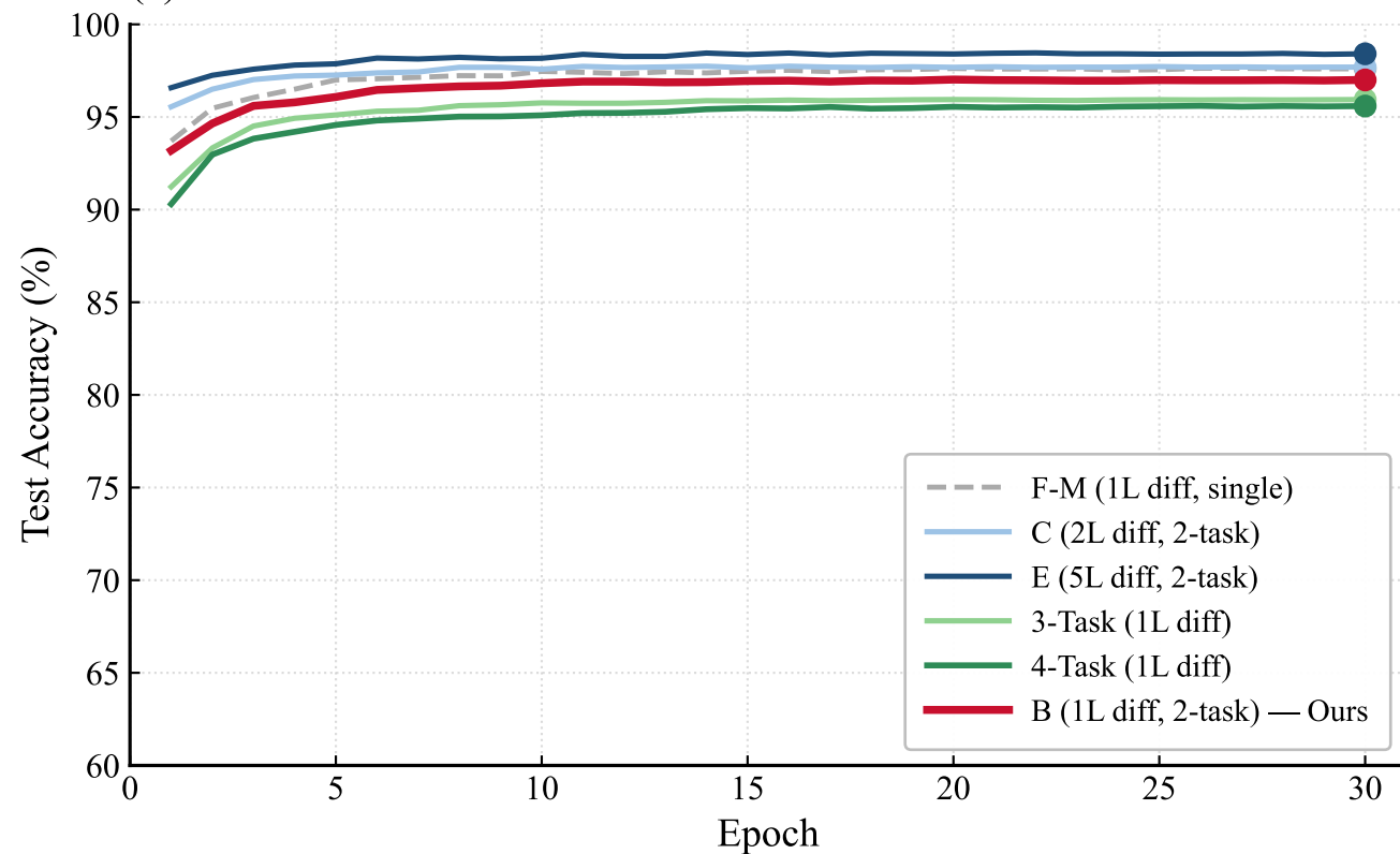
(c) Fashion-MNIST — Differential
