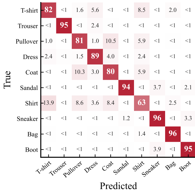
Fashion-MNIST (87.12%)
