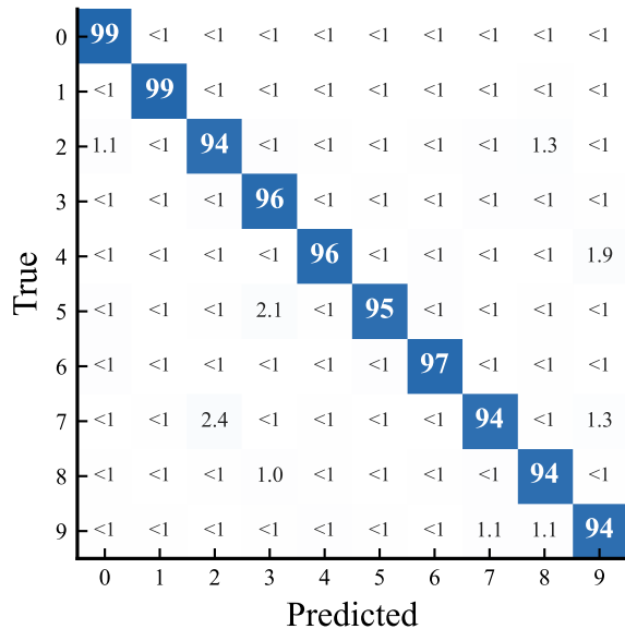
MNIST (95.94%)
