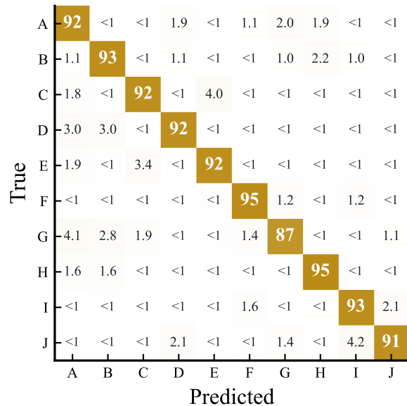
EMNIST (A-J) (92.28%)
