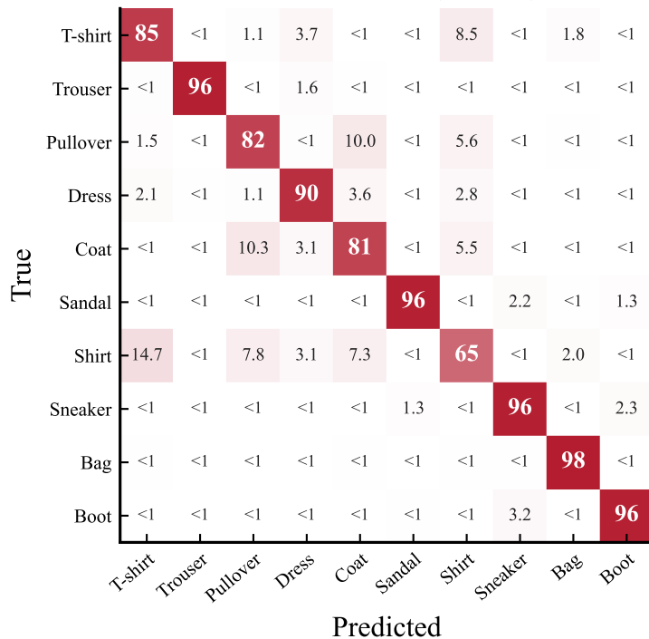
Fashion-MNIST (88.38%)
