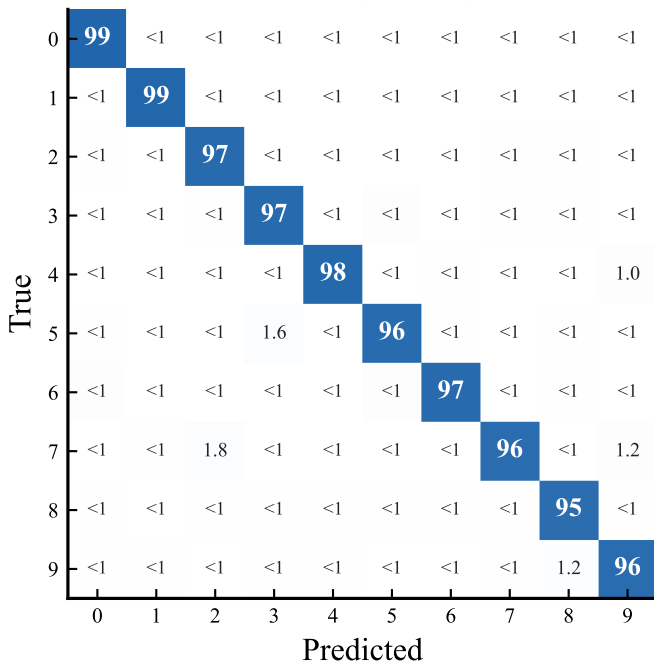
MNIST (97.00%)
