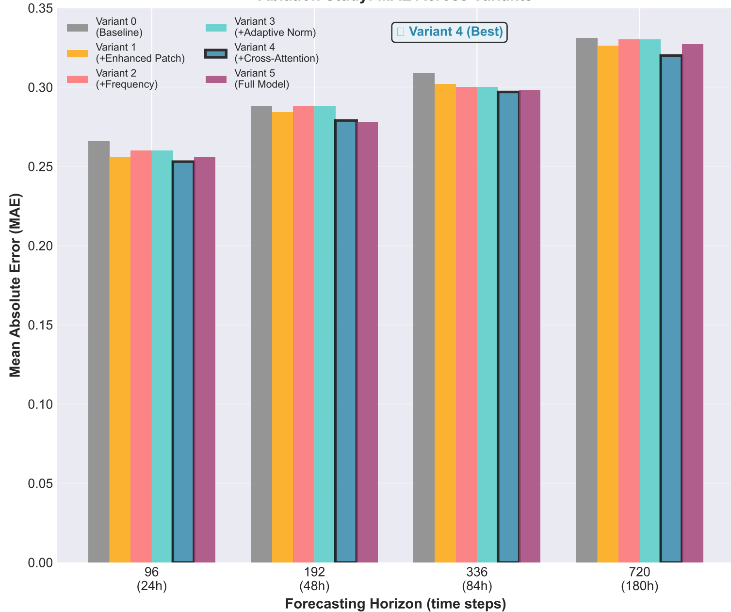
Ablation Study: MAE Across Variants
