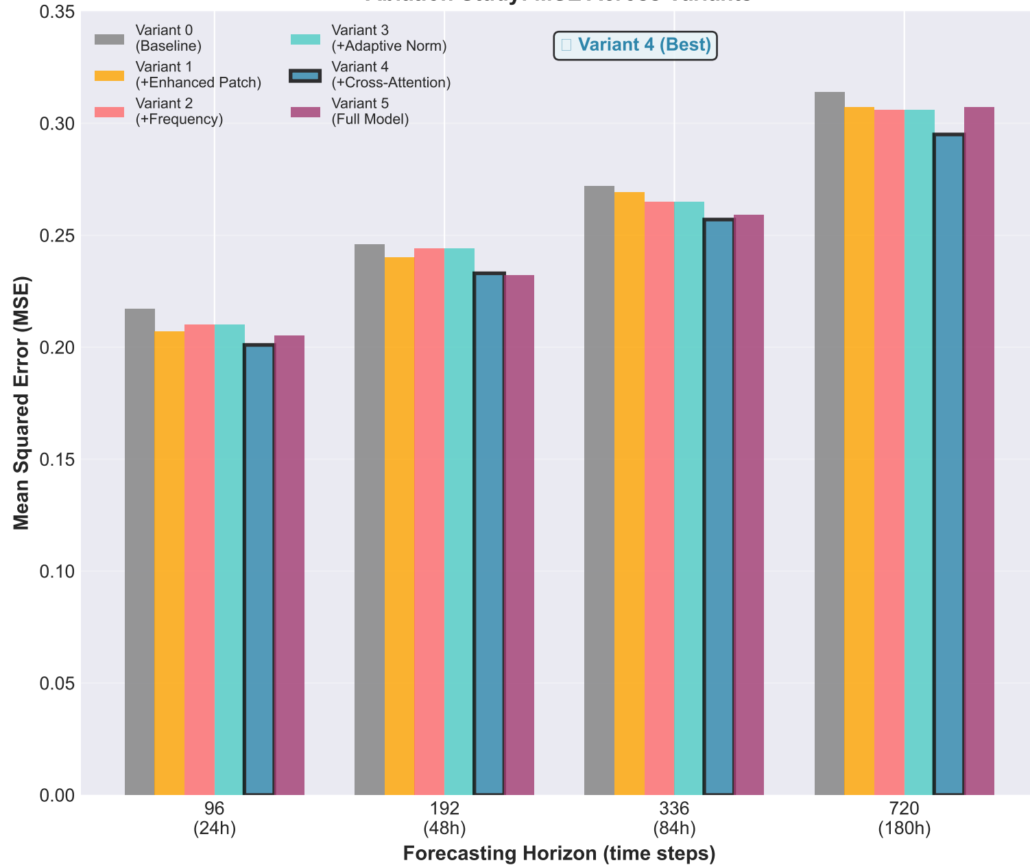
Ablation Study: MSE Across Variants
