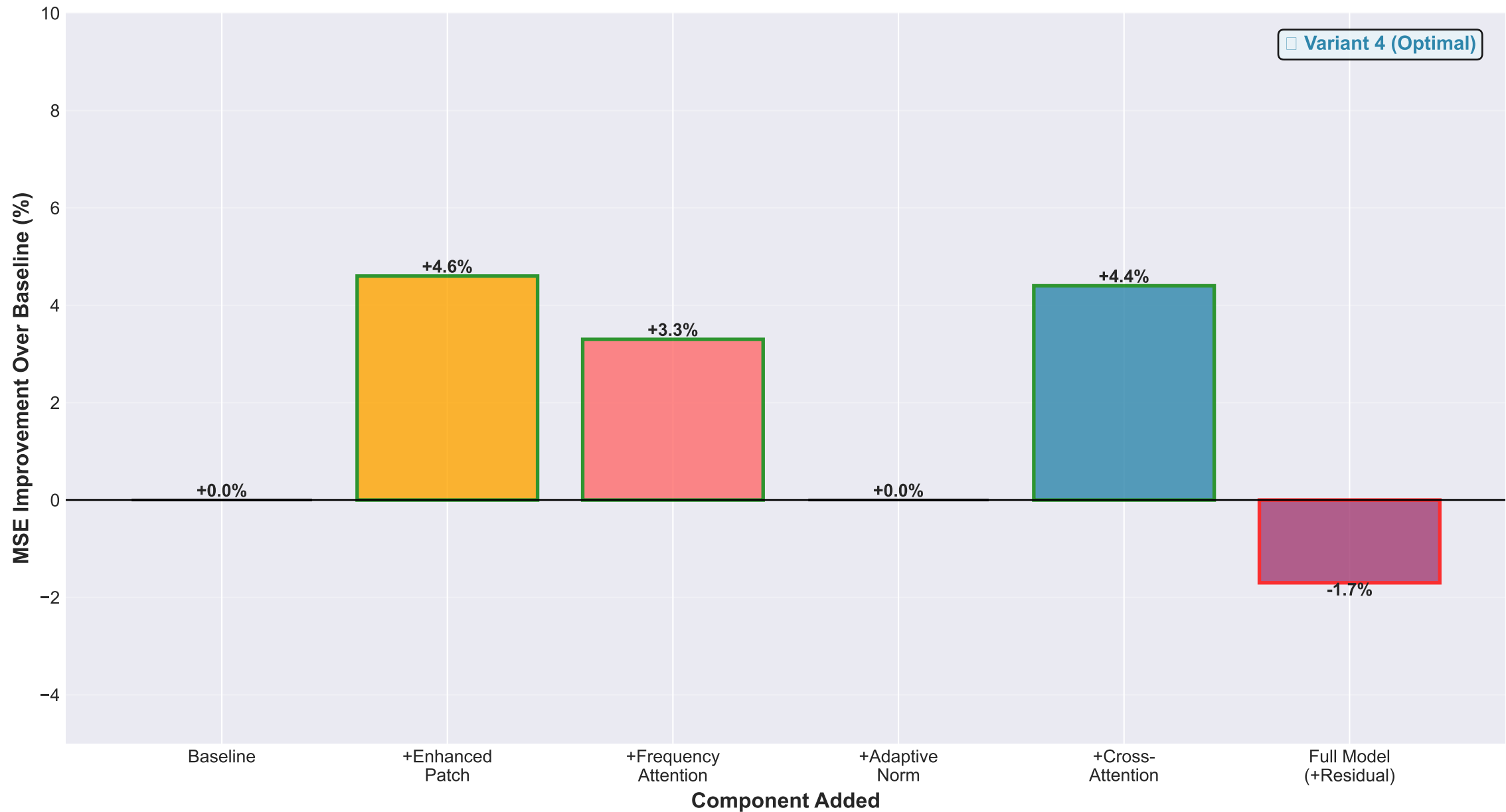
Component Contribution Analysis (96-step Horizon)
