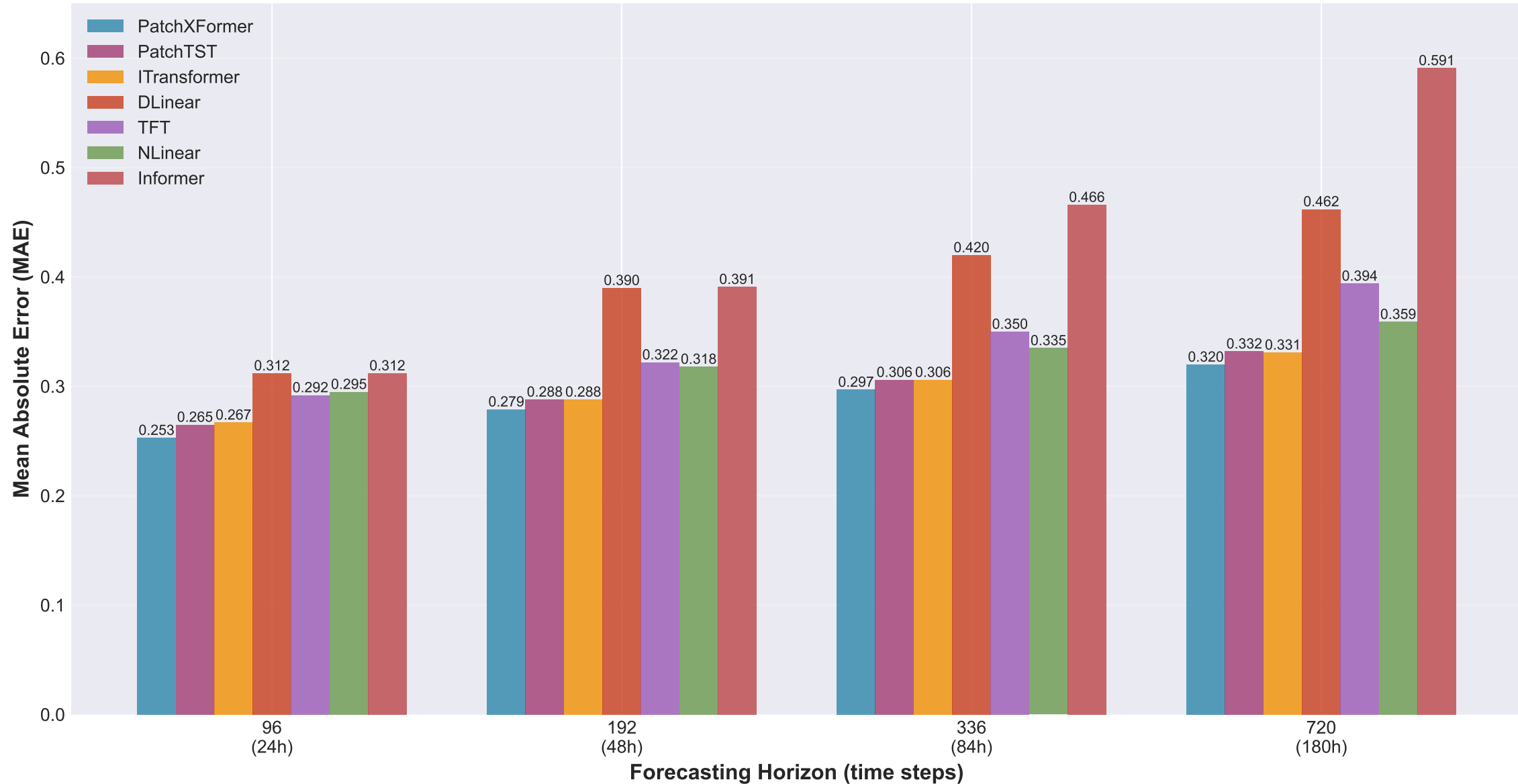
Model Comparison: MAE Across Forecasting Horizons (Piliyandala Dataset)
