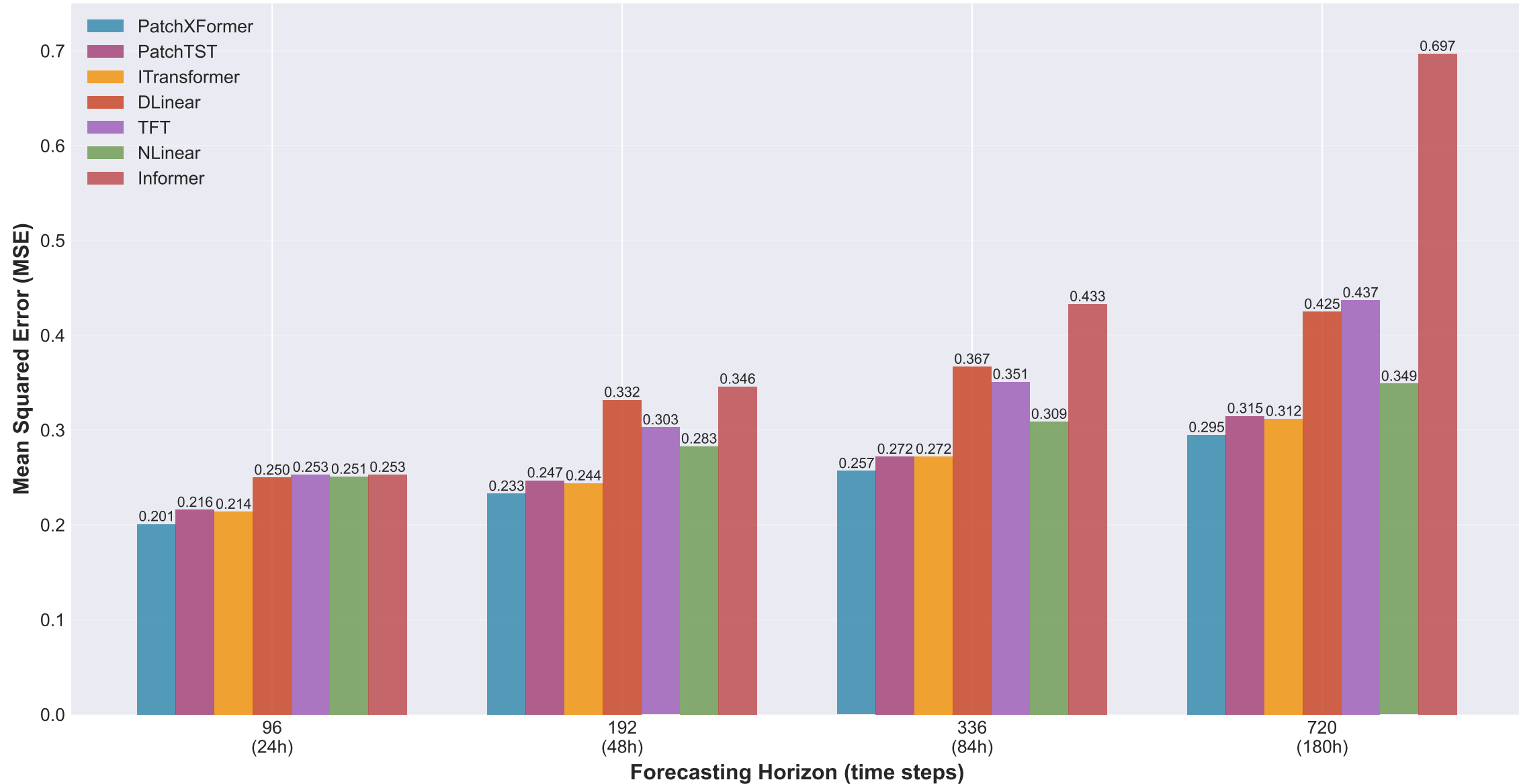
Model Comparison: MSE Across Forecasting Horizons (Piliyandala Dataset)
